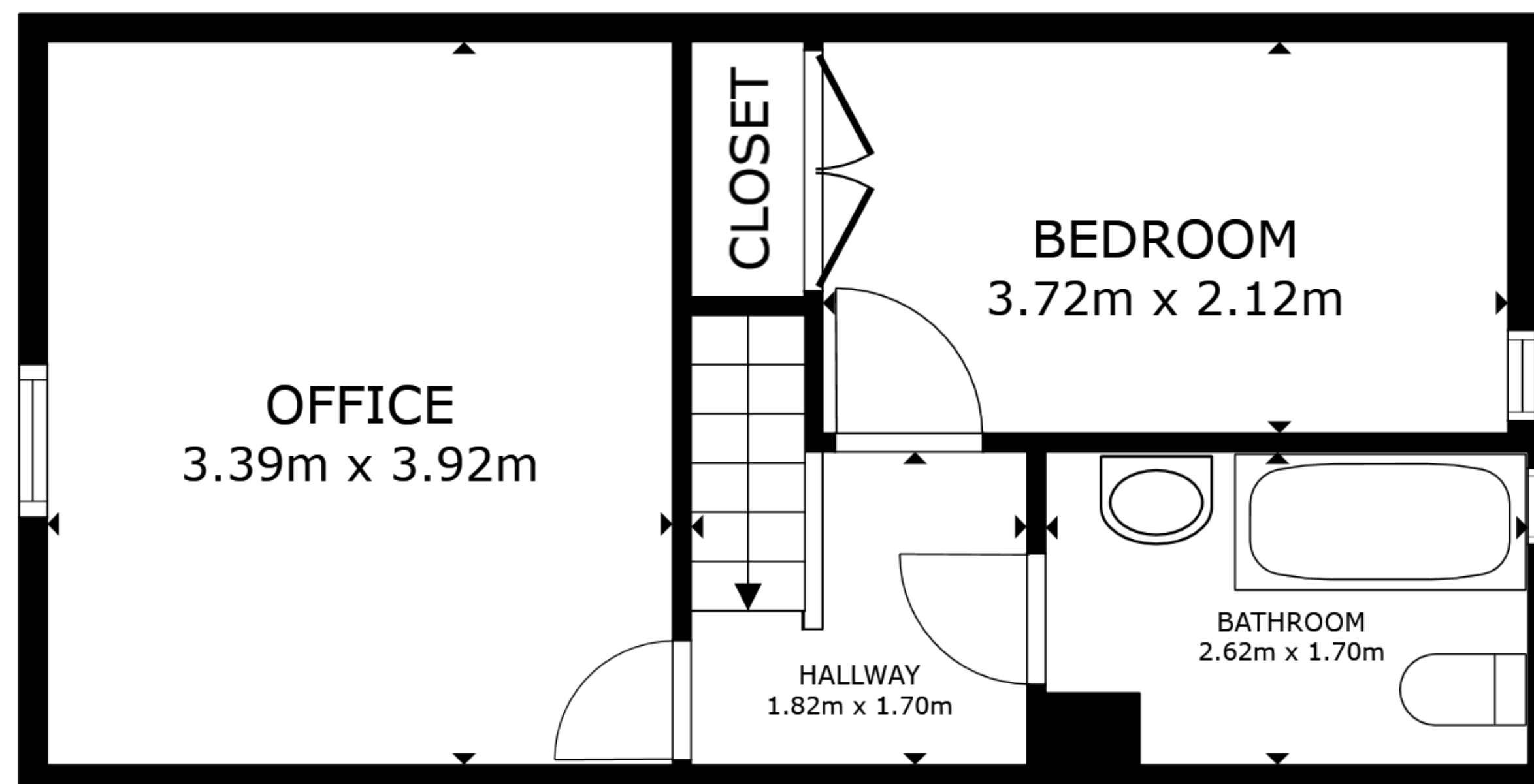
FLOOR 2
