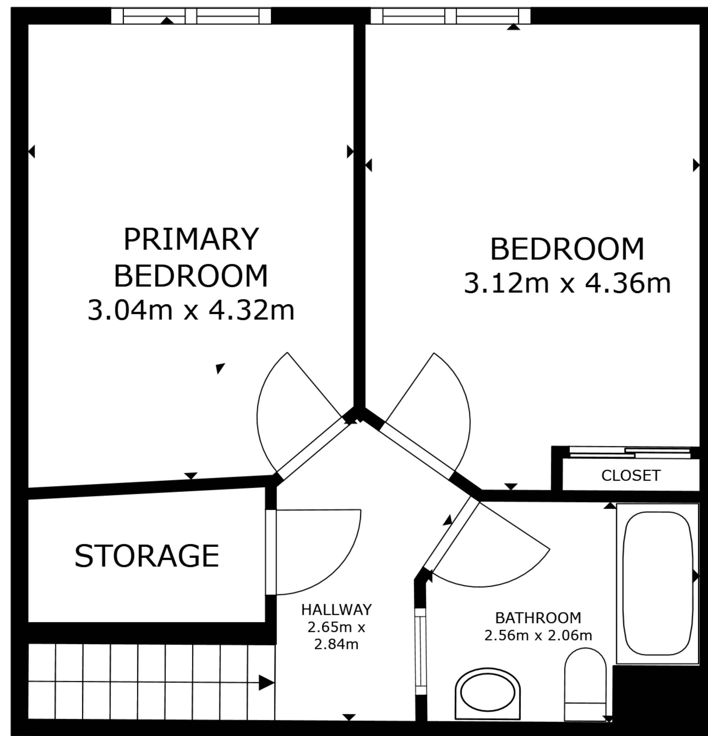
FLOOR 2
