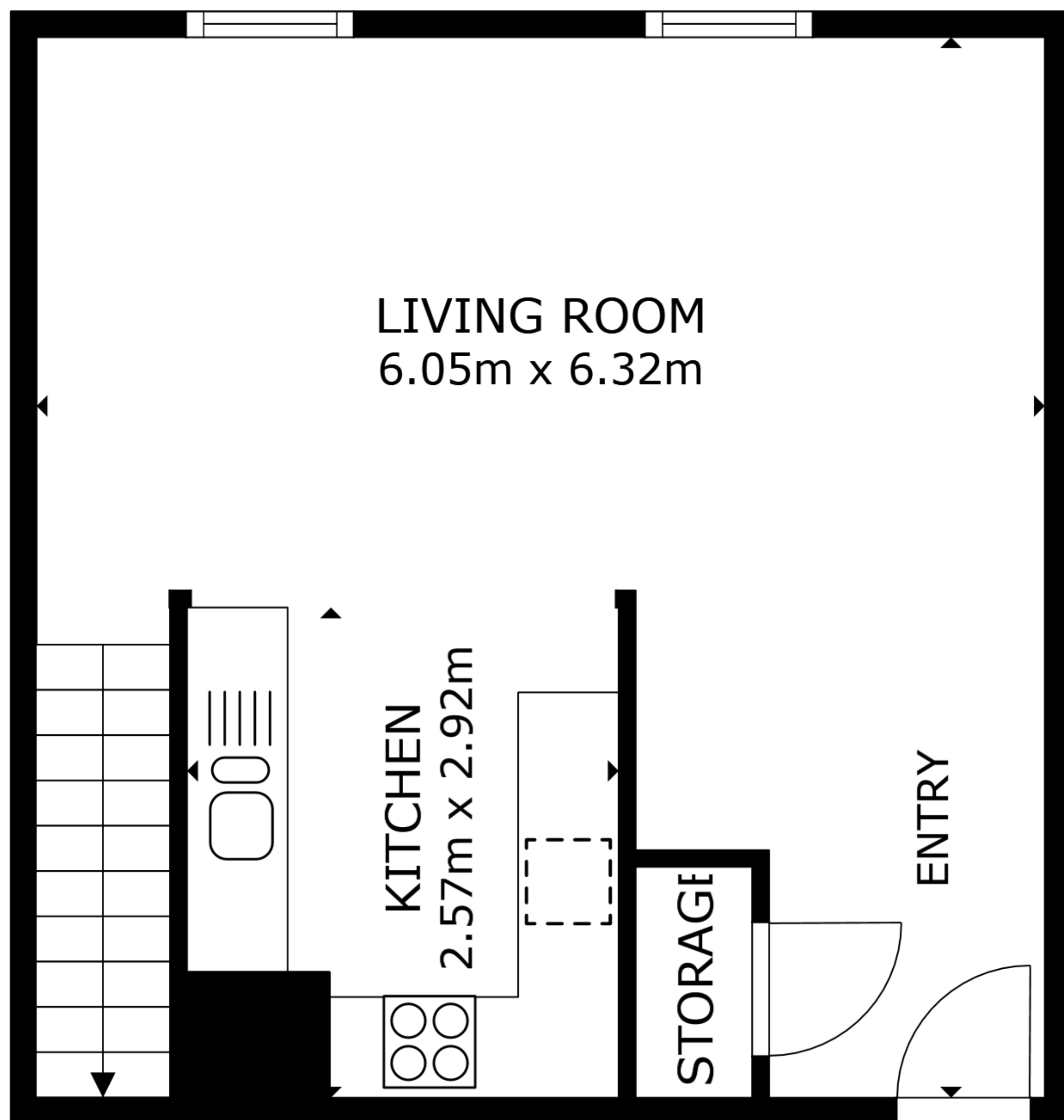
FLOOR 1
