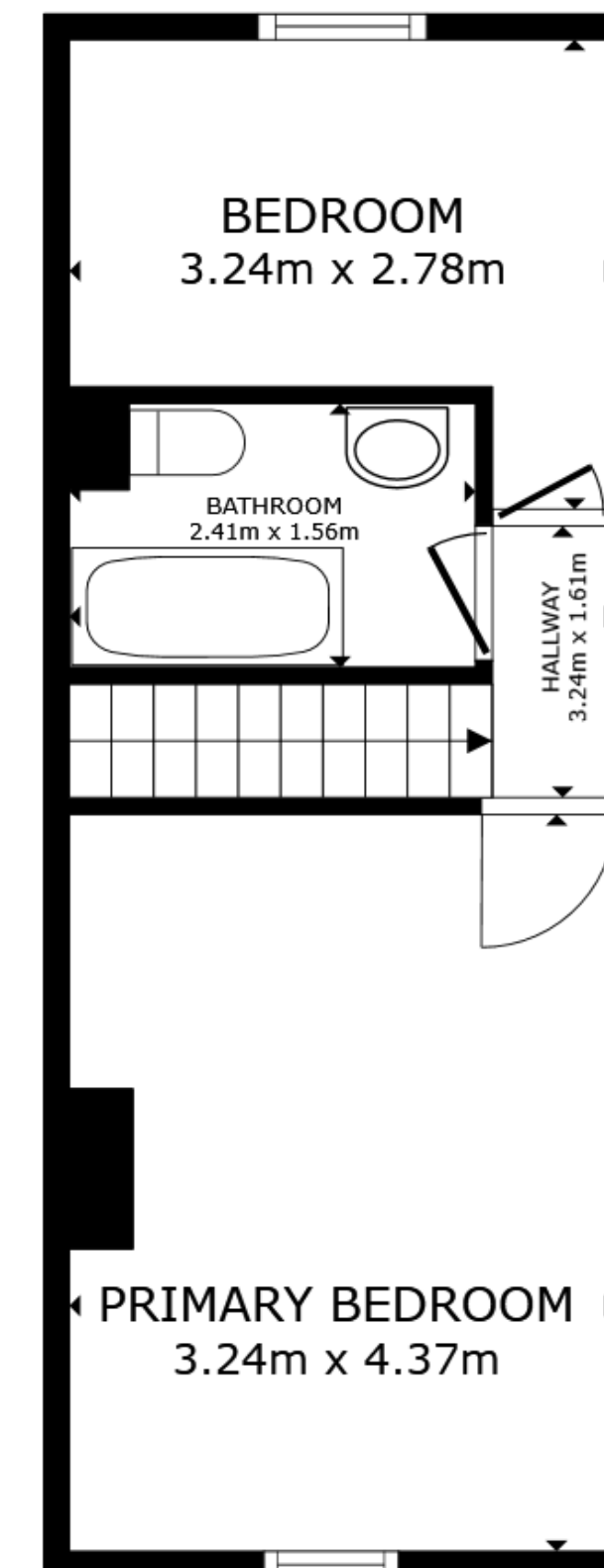
FLOOR 2
