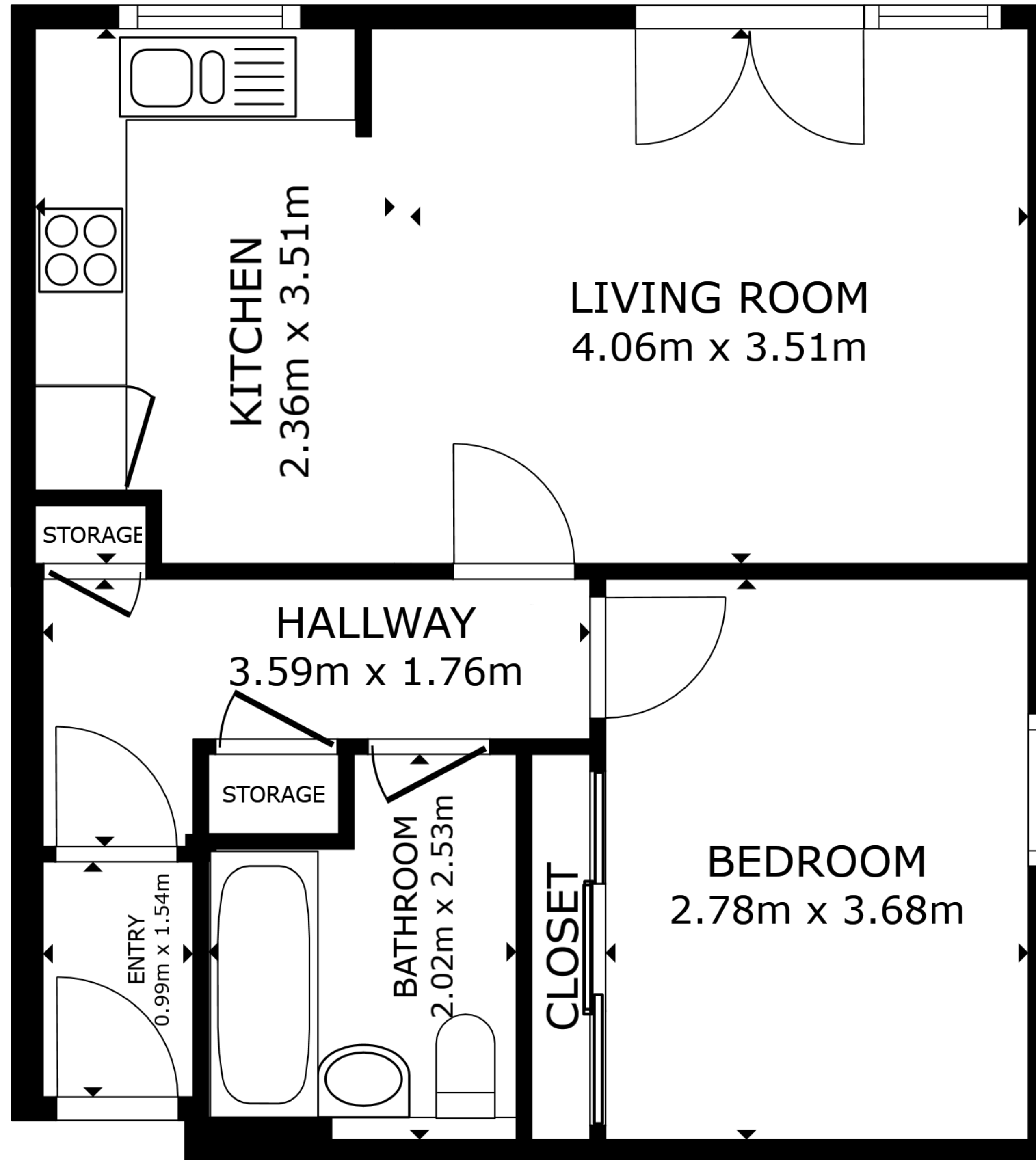
FLOOR PLAN
