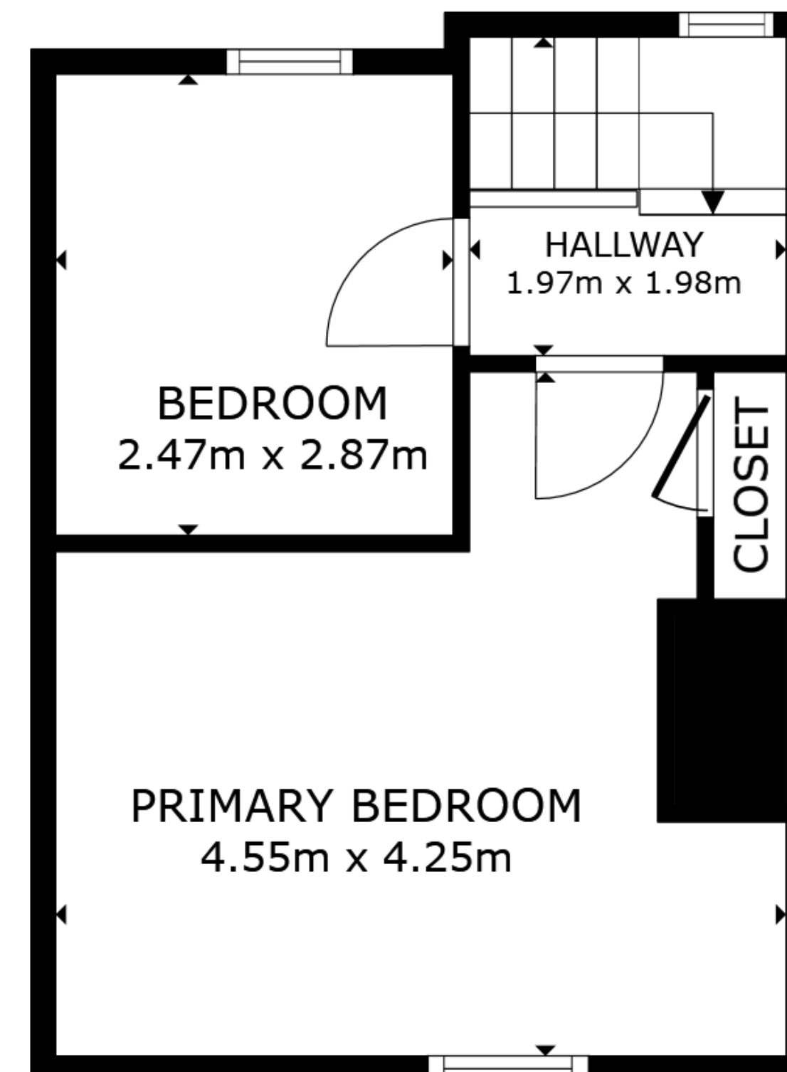
FLOOR 2
