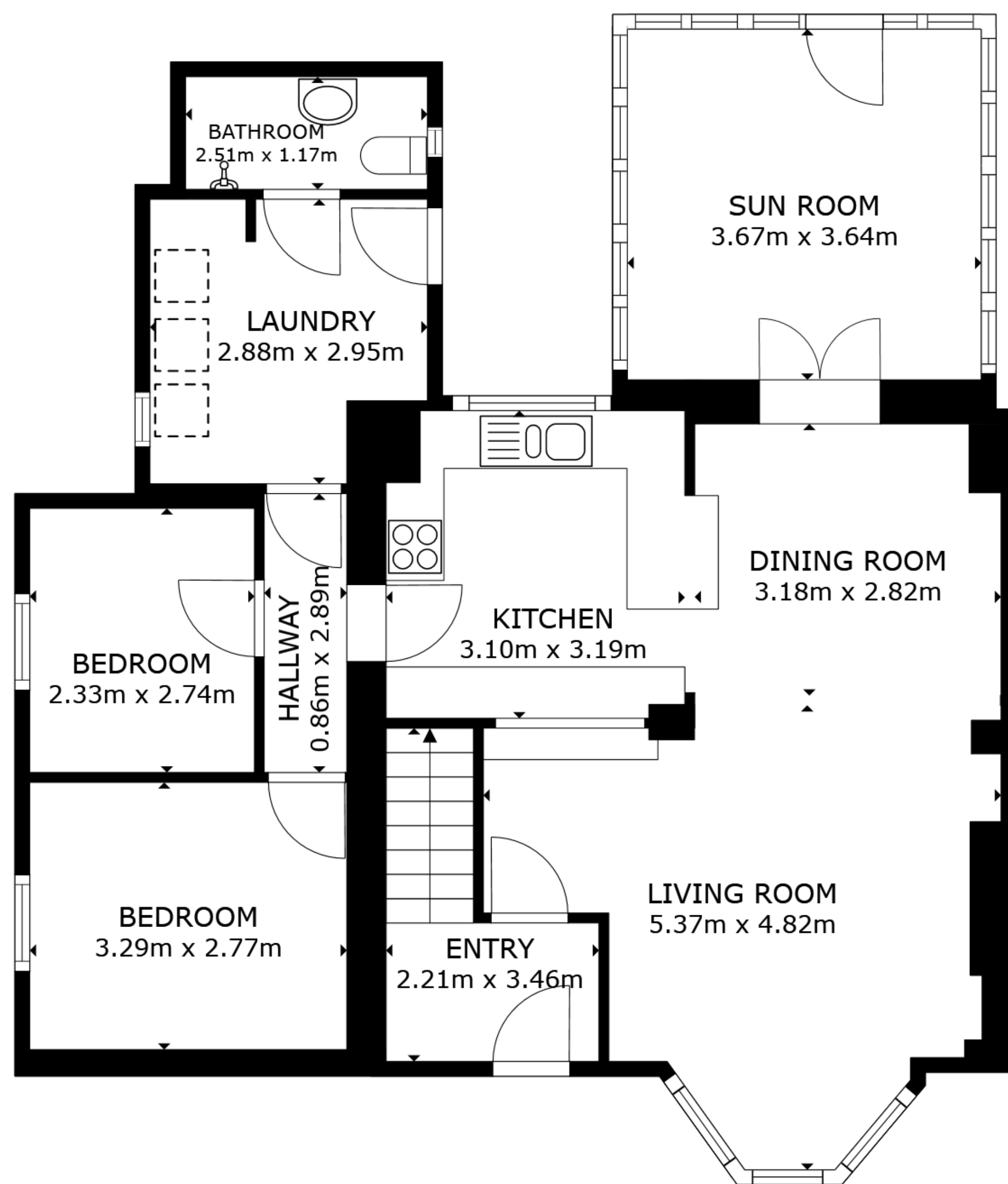
FLOOR 1
