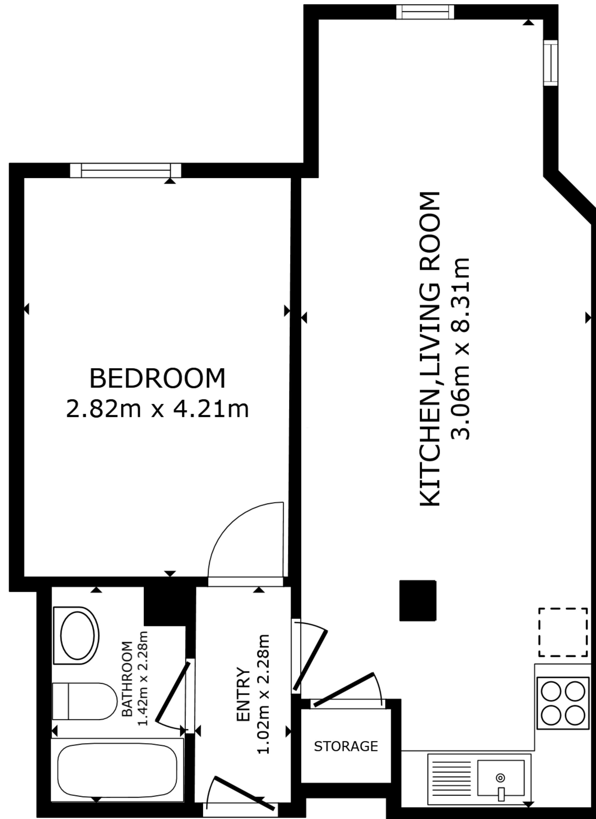
FLOOR PLAN
