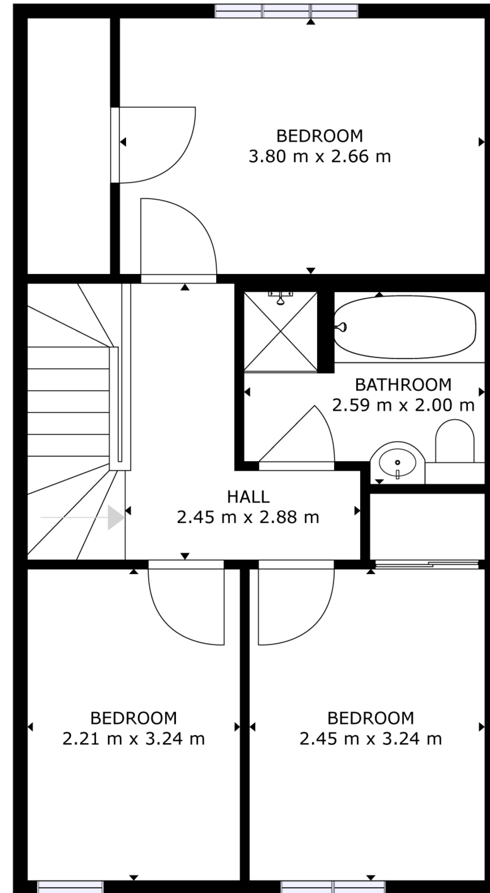
FLOOR 2
