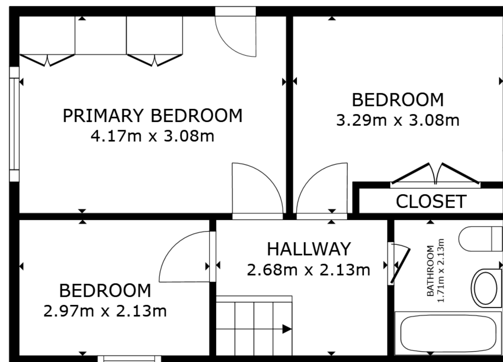
FLOOR 2
