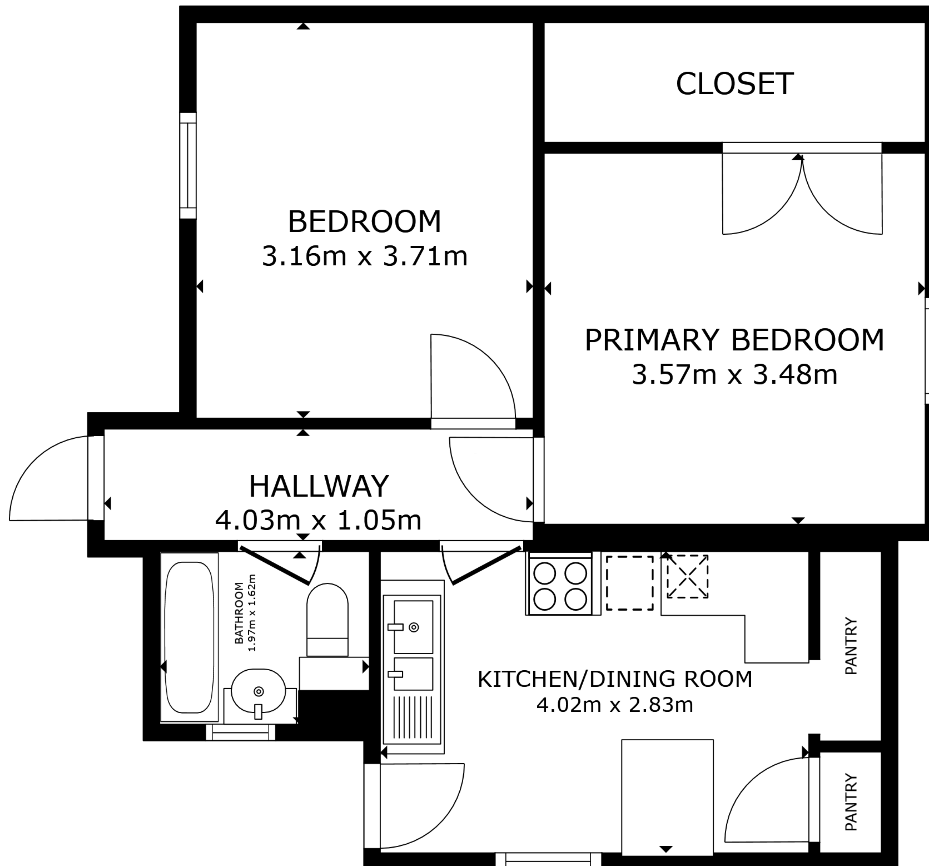
FLOOR PLAN
