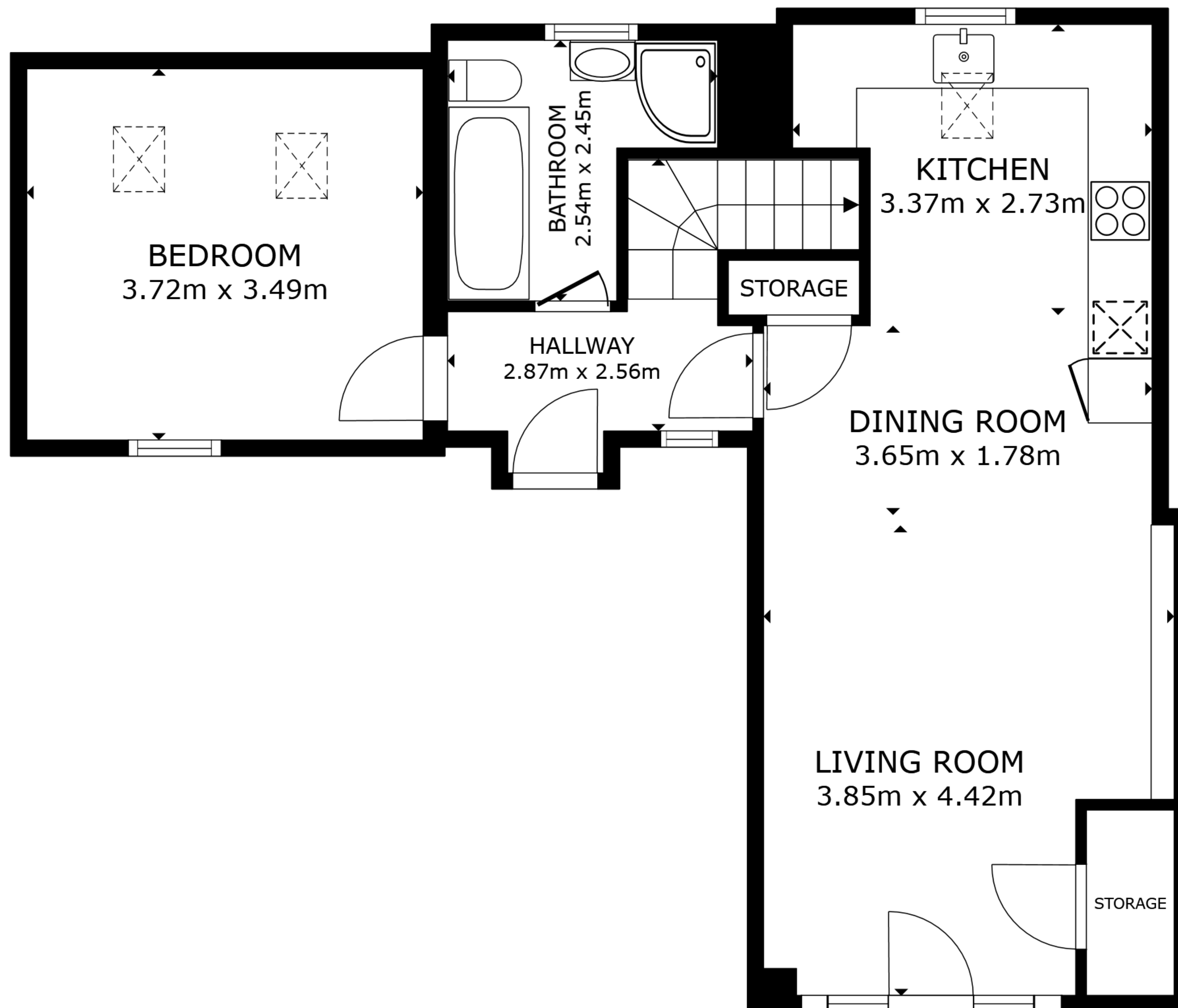
FLOOR 1
