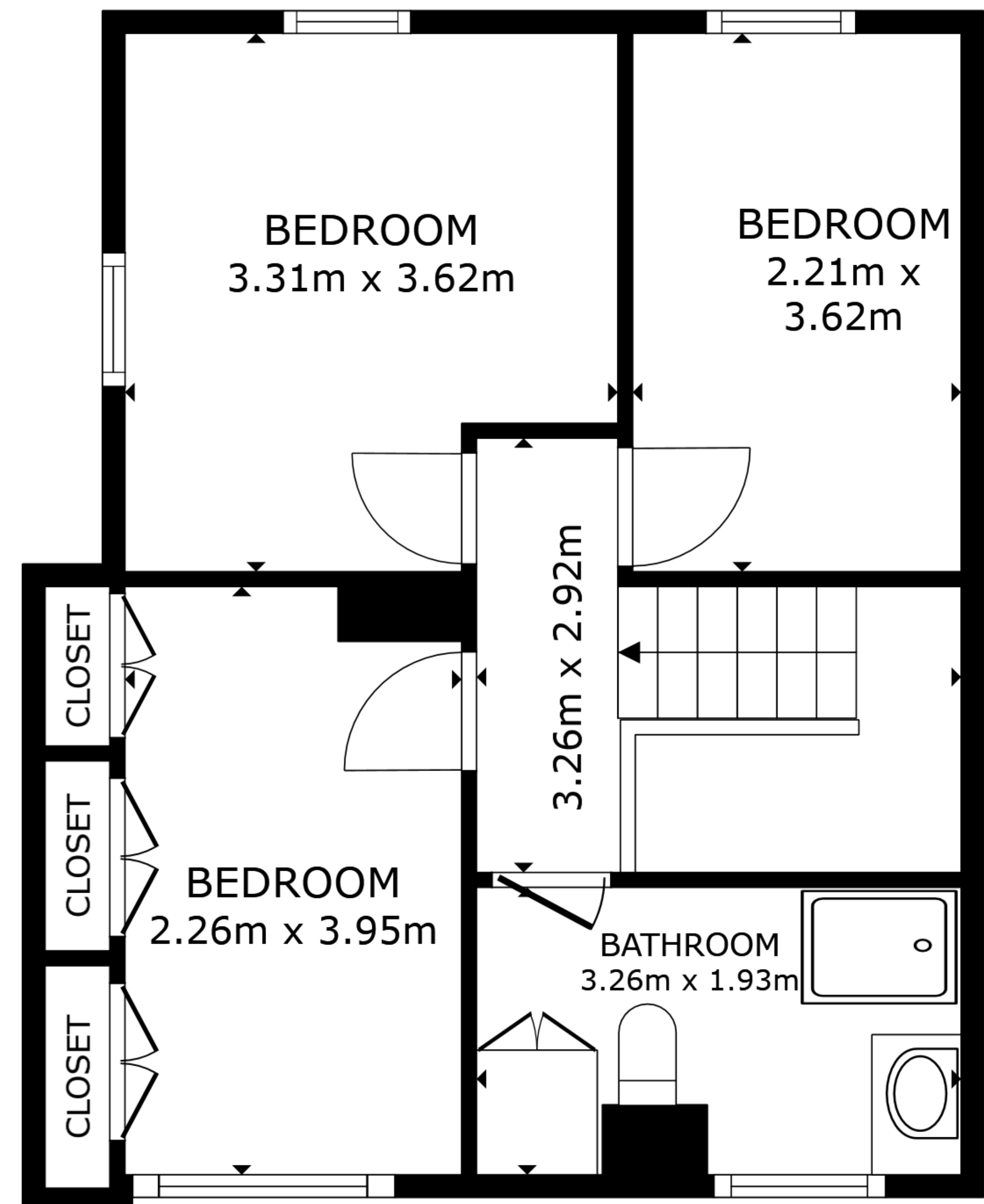
FLOOR 2
