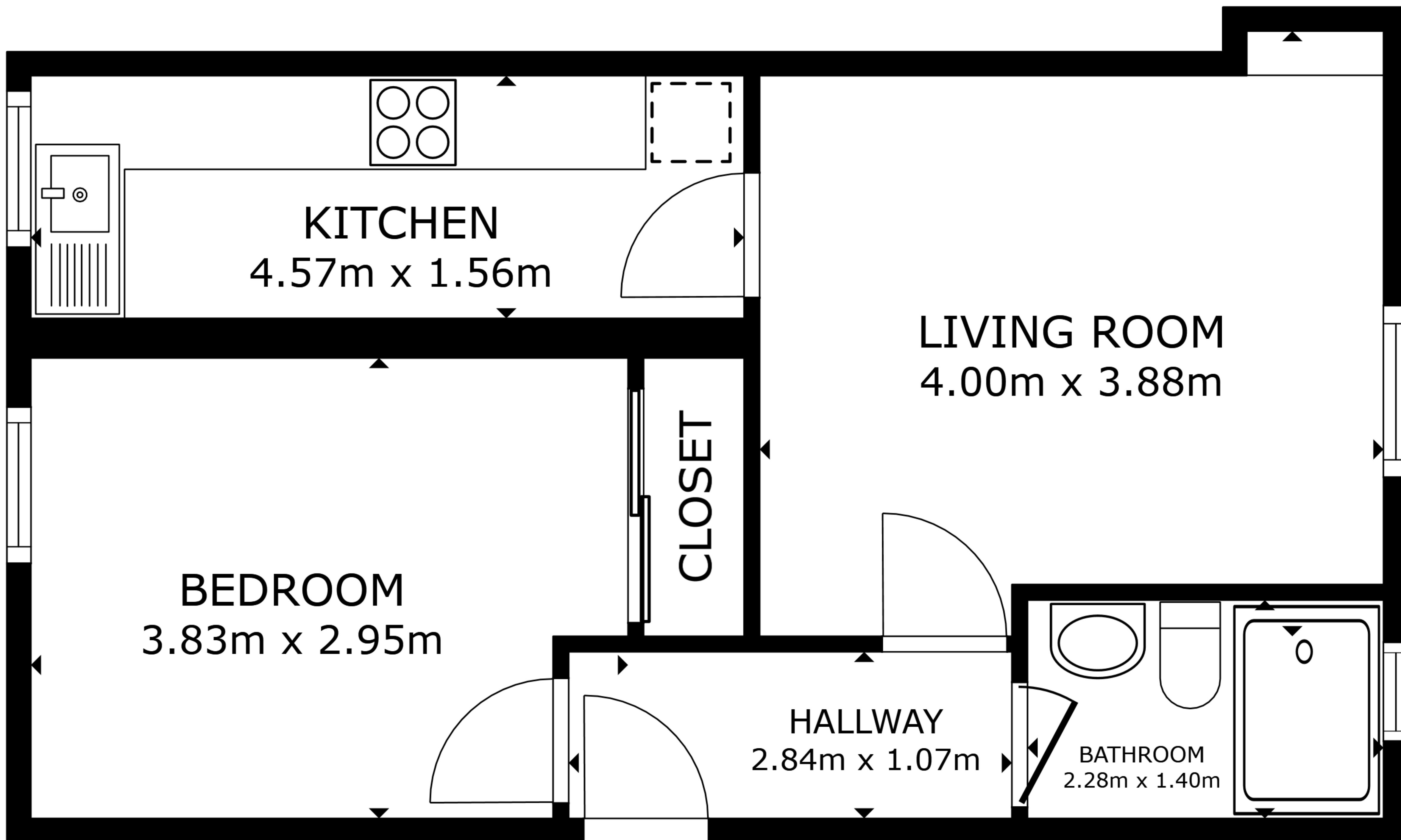
FLOOR PLAN
