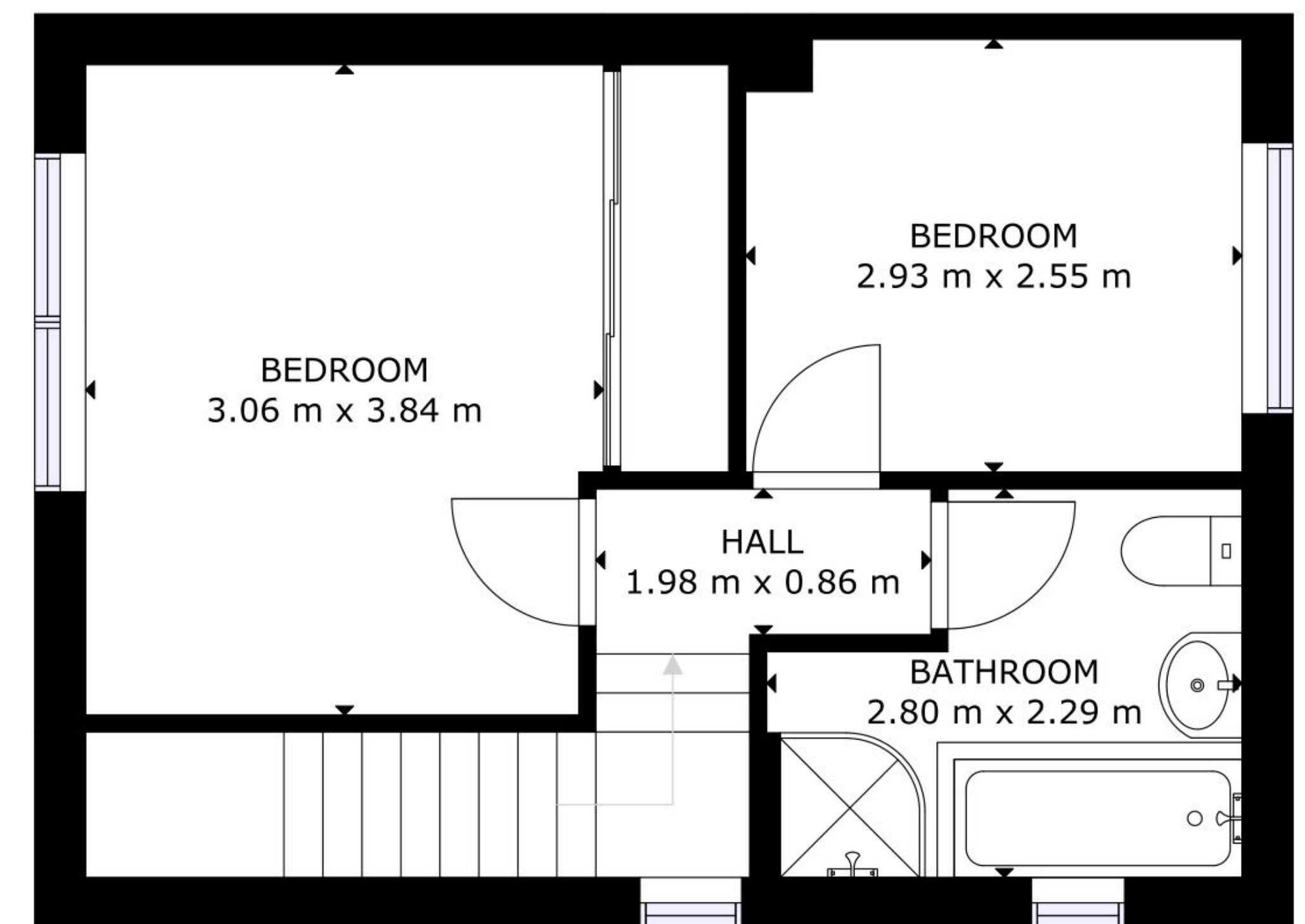
FLOOR 2
