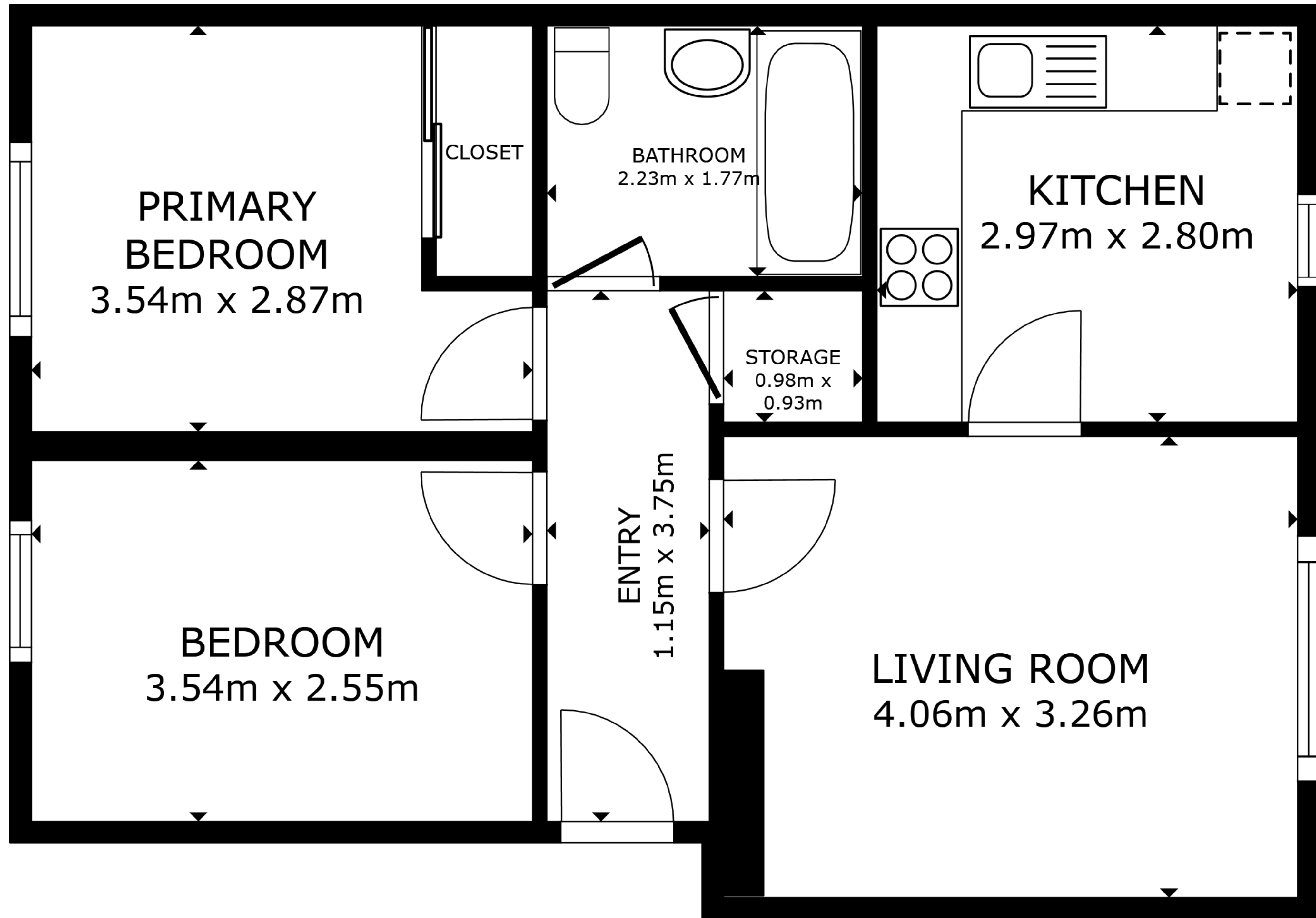
FLOOR PLAN
