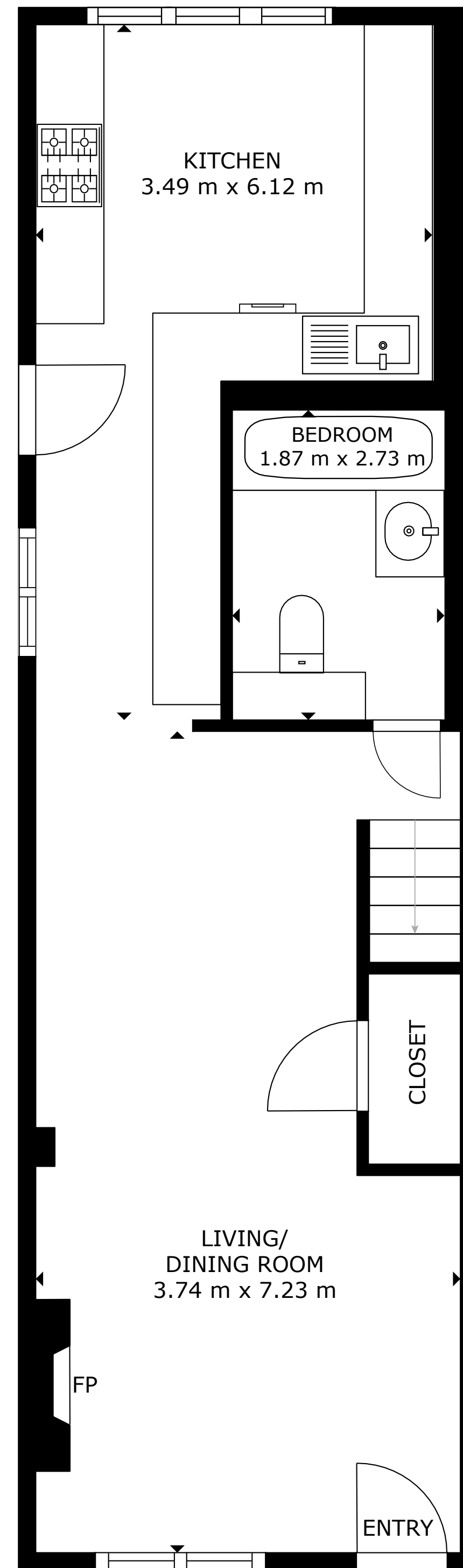
FLOOR 1
