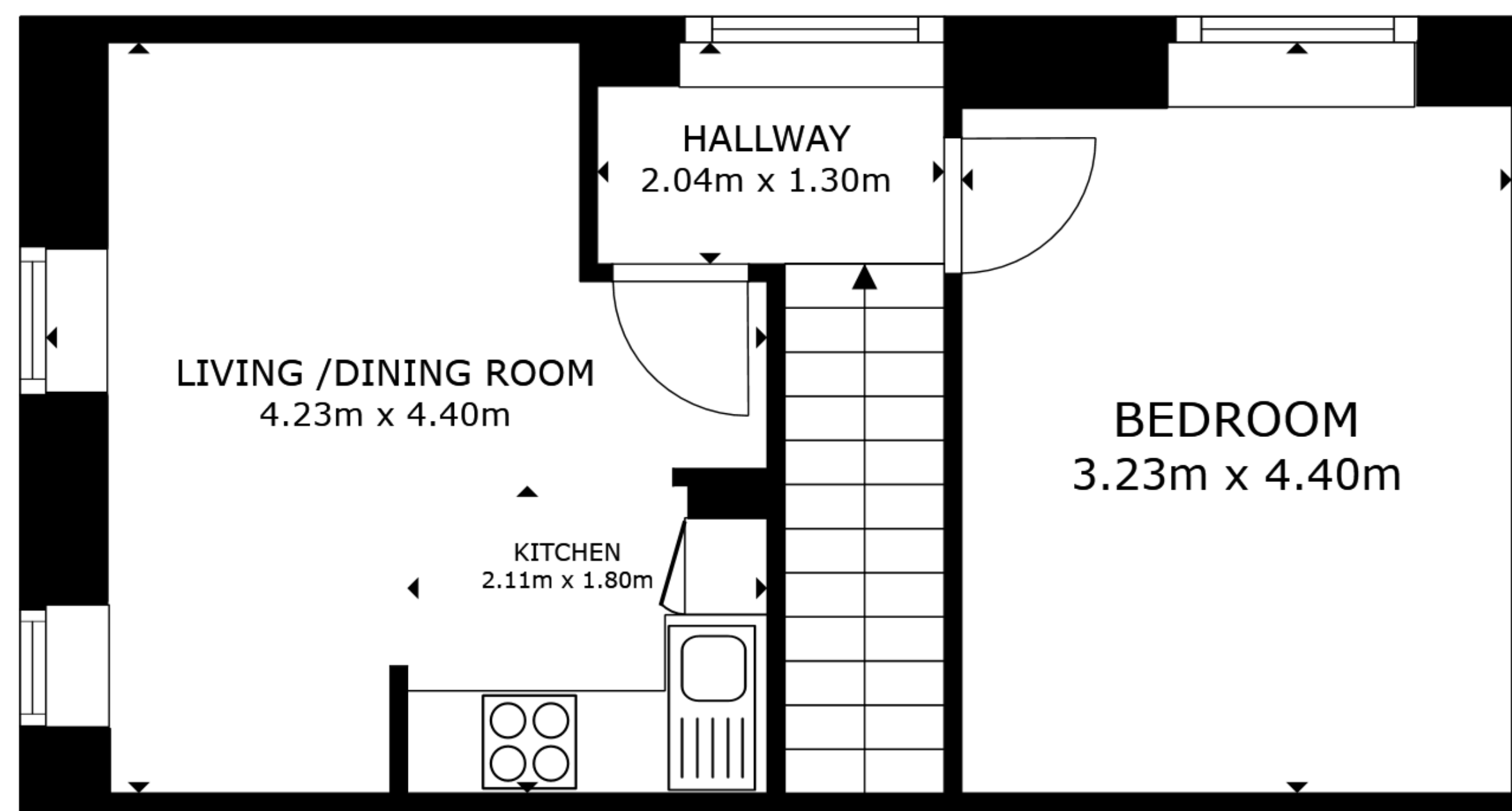
FLOOR 2
