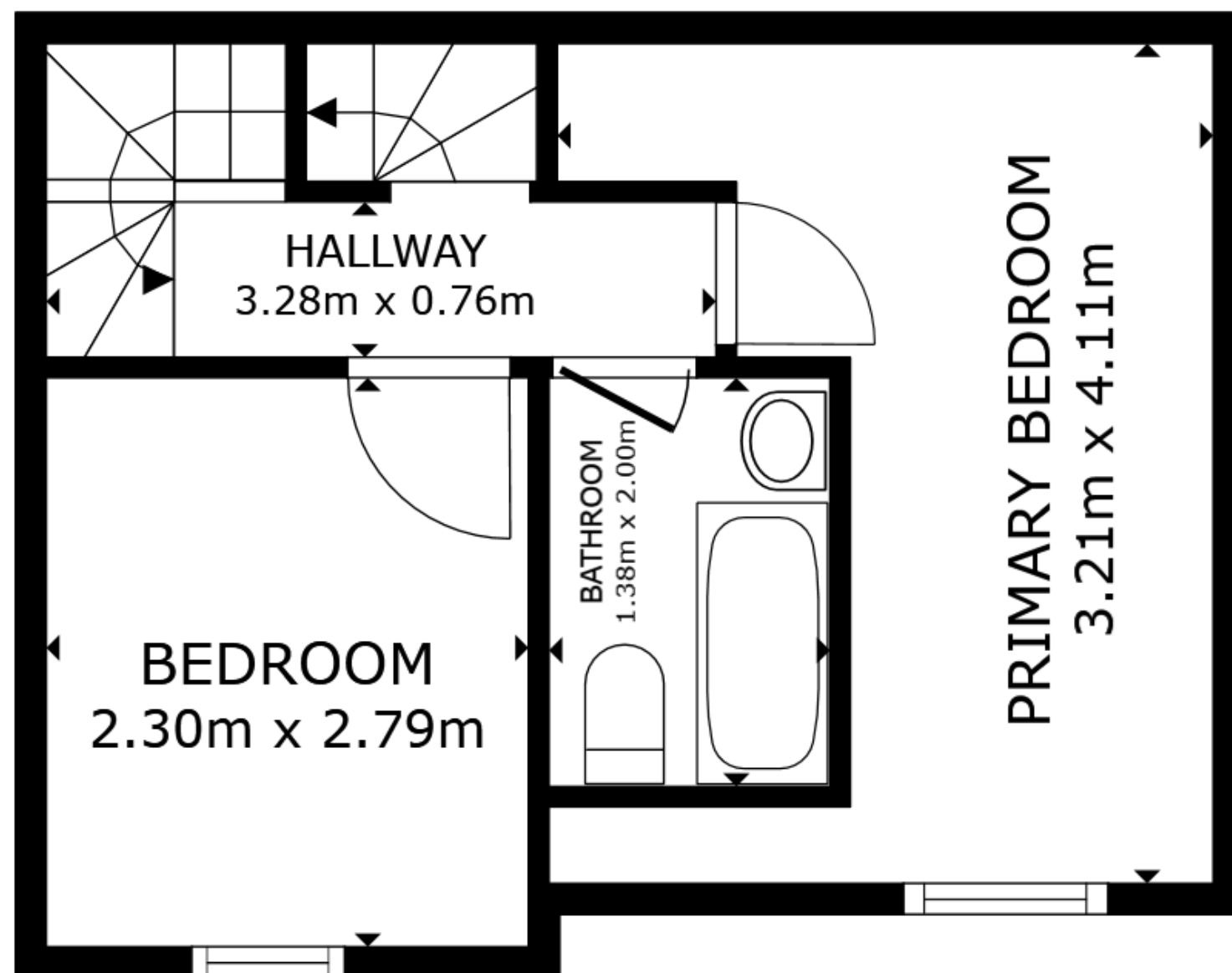
FLOOR 1
