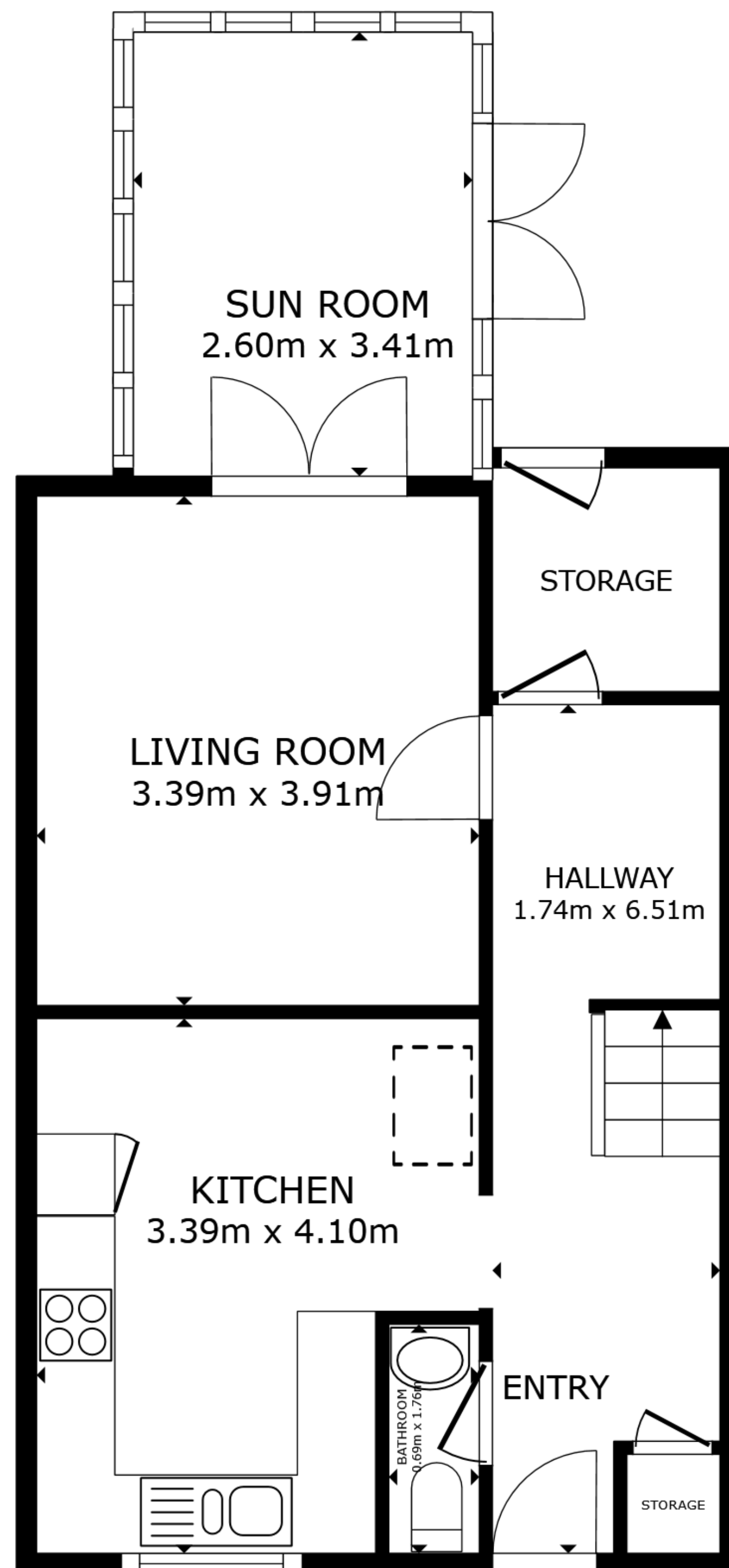
FLOOR 1
