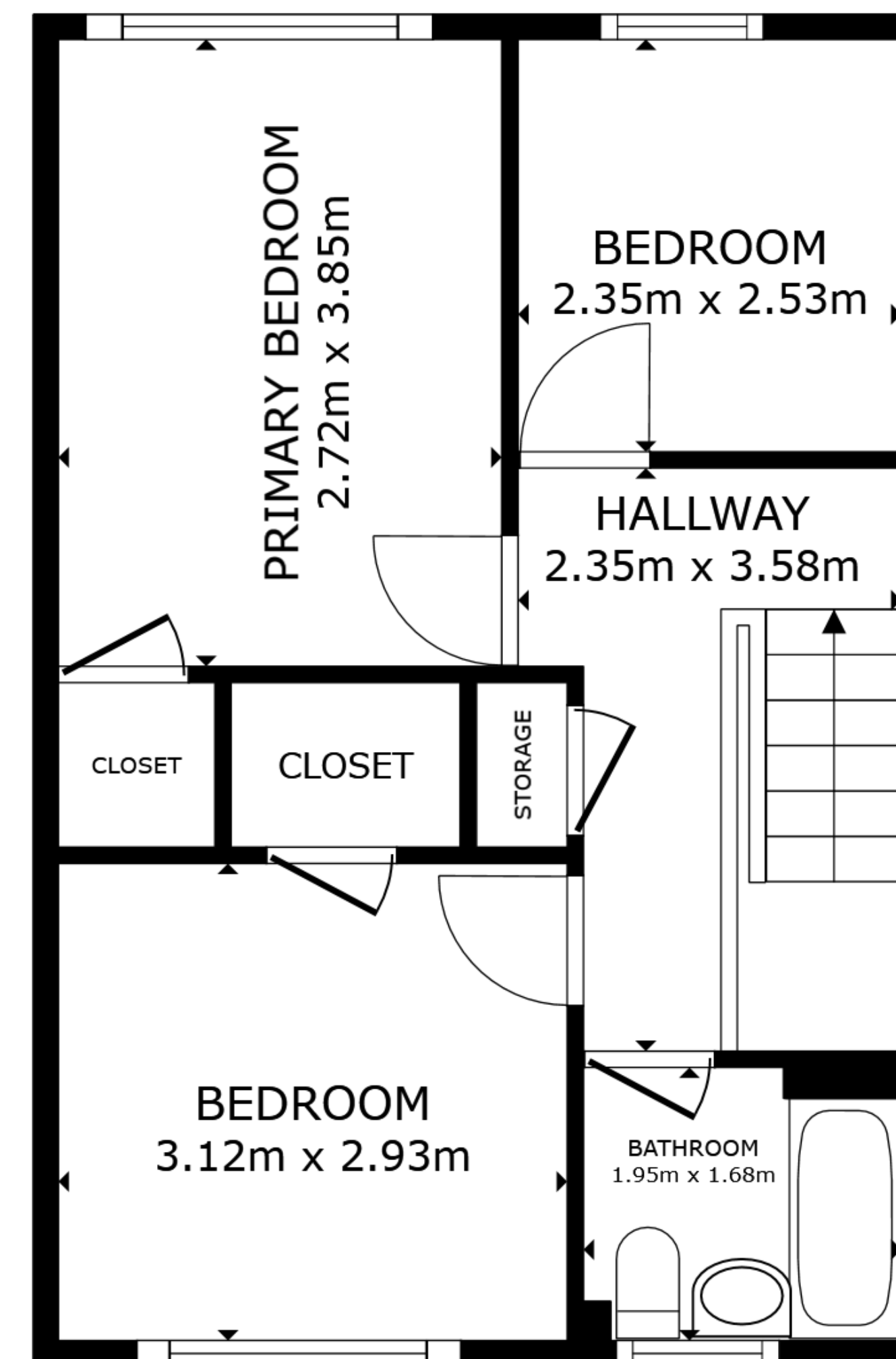
FLOOR 2
