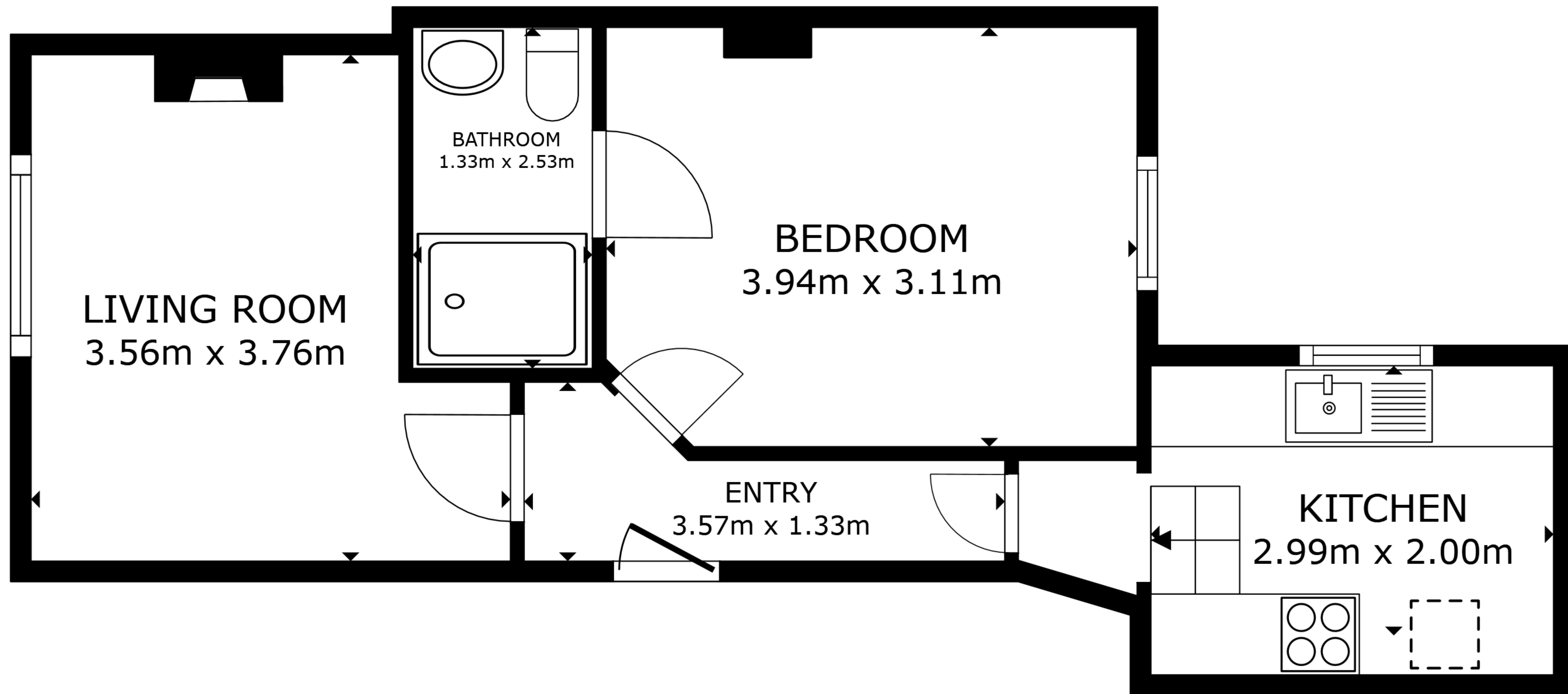
FLOOR PLAN
