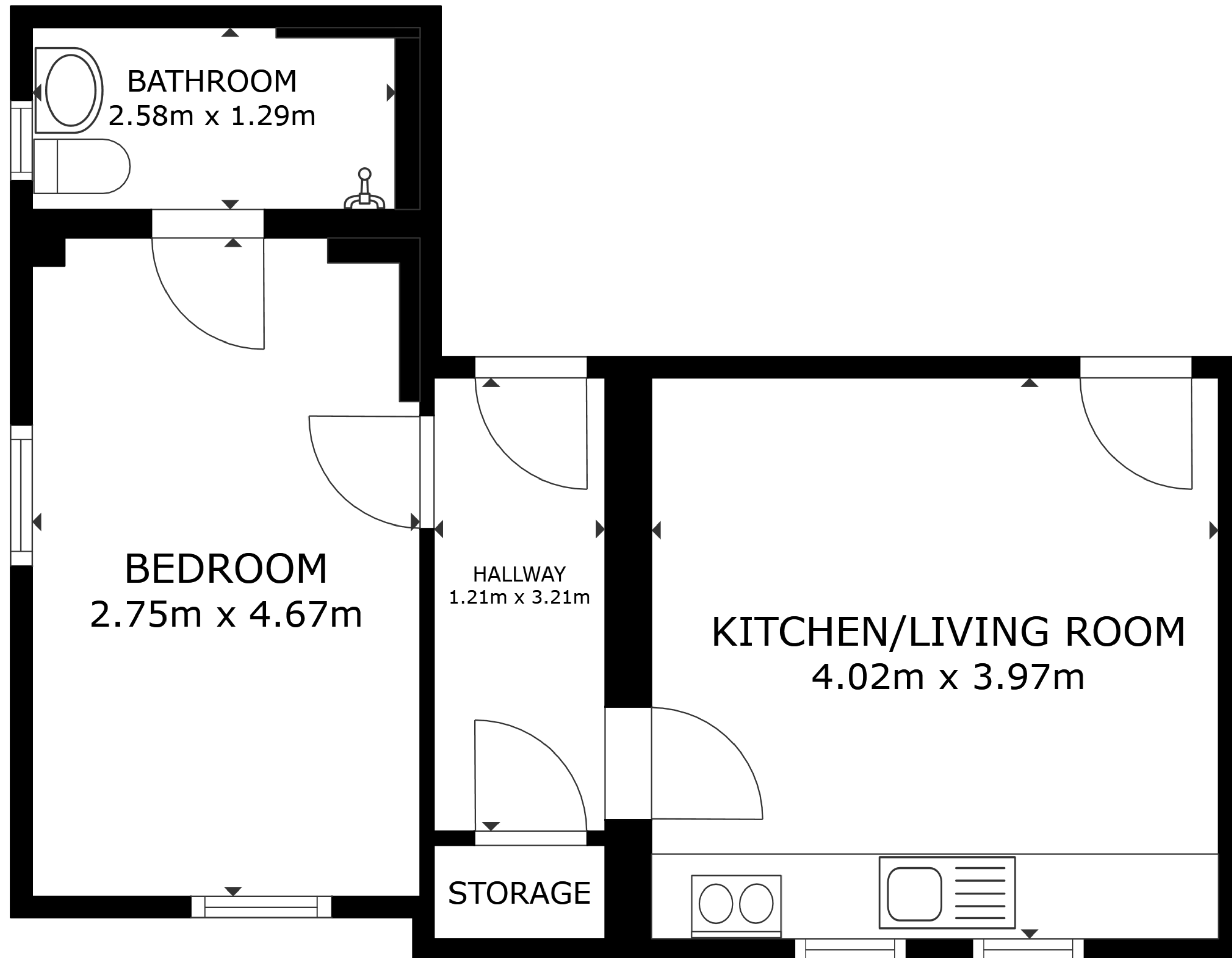
FLOOR PLAN
