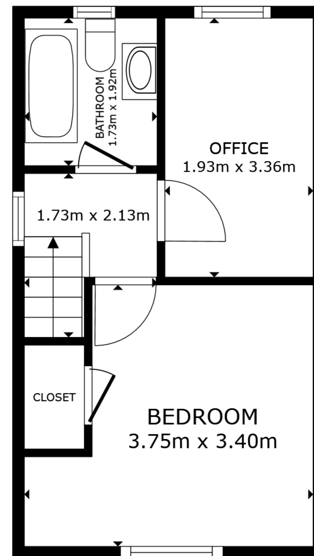
FLOOR 2
