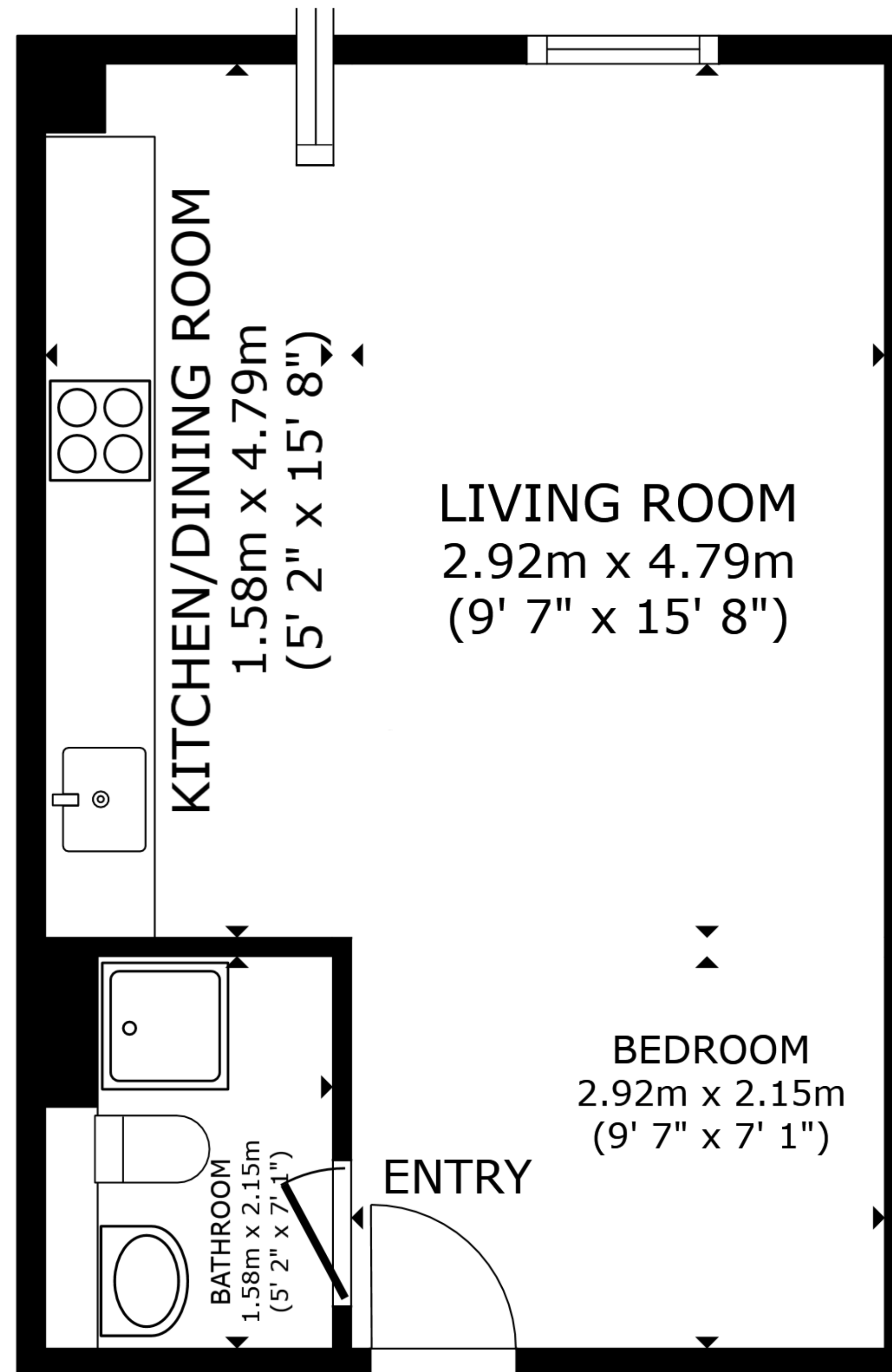
FLOOR PLAN
