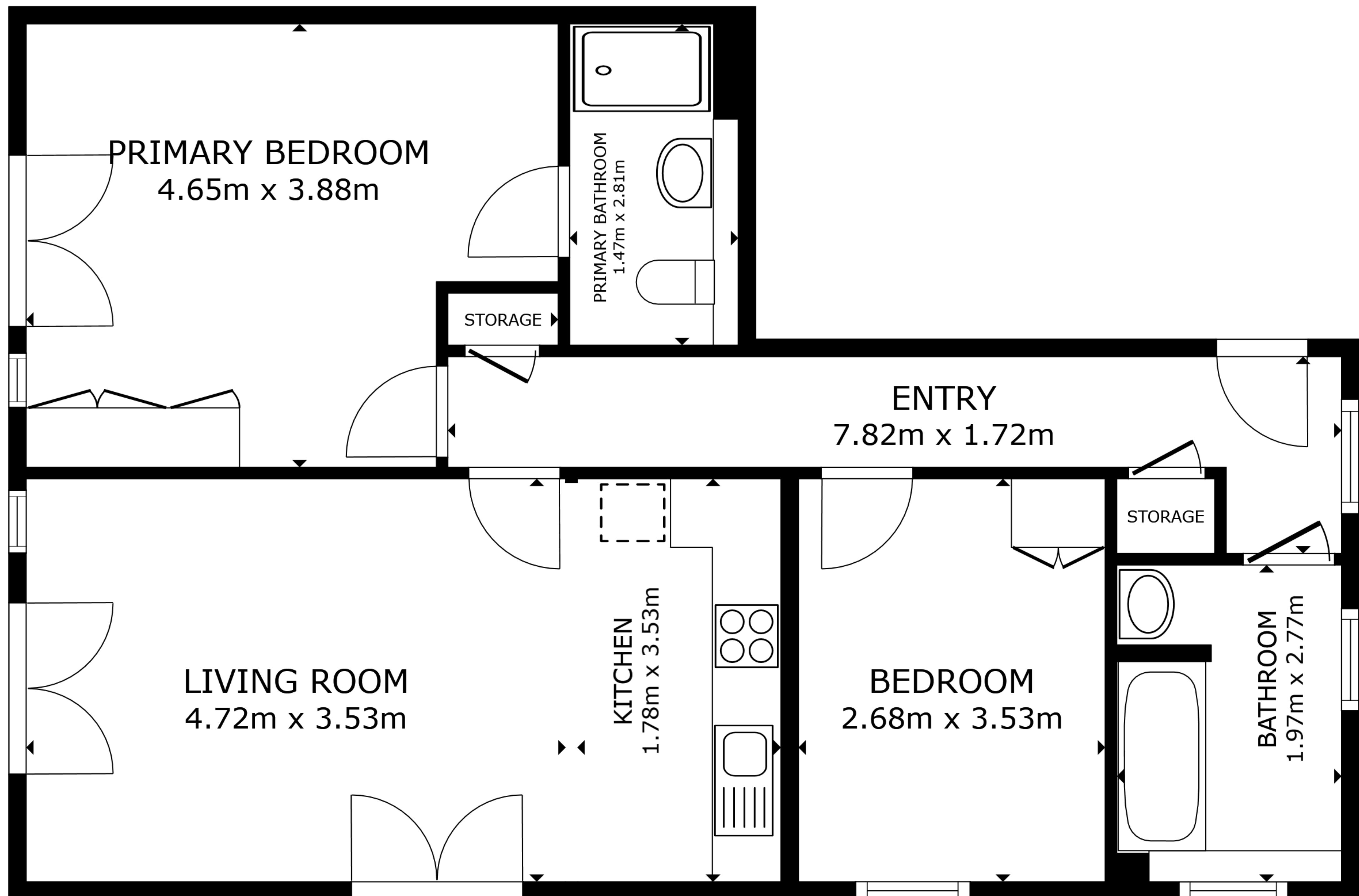
FLOOR PLAN
