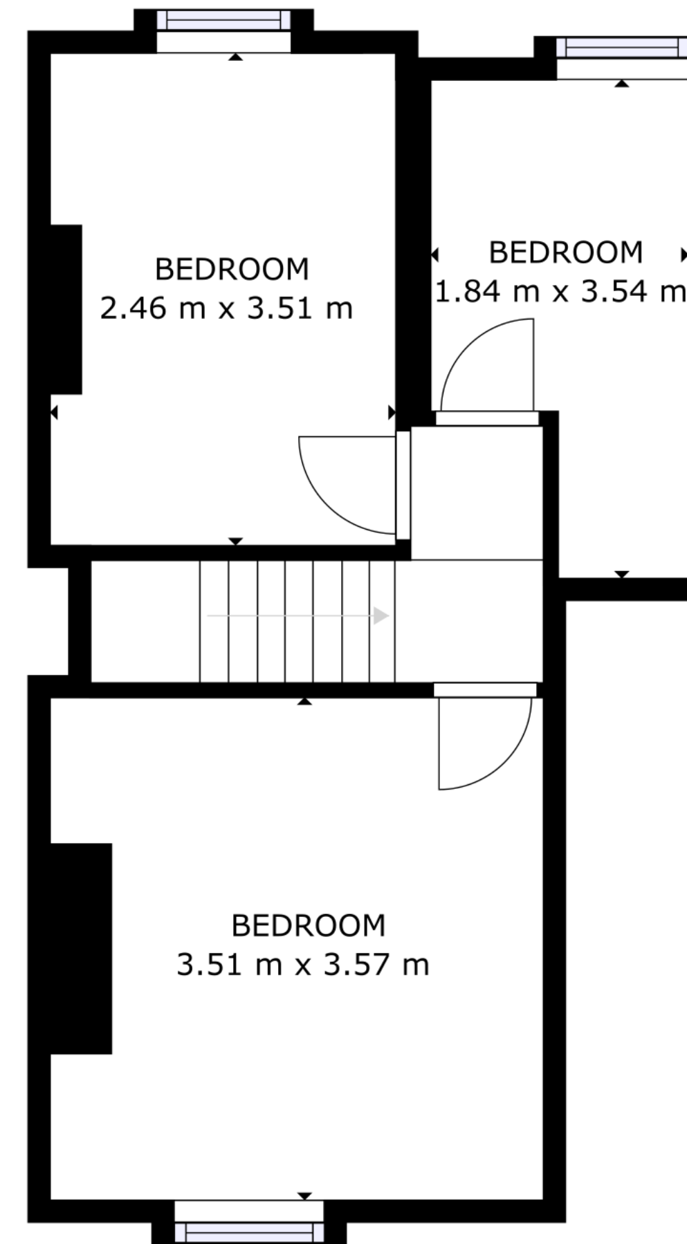
FLOOR 2
