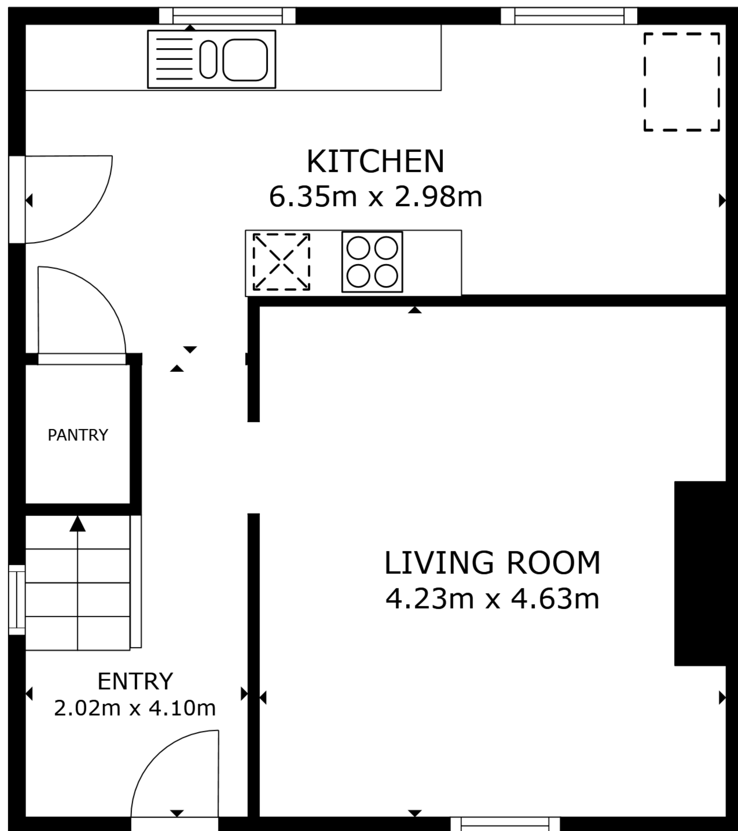
FLOOR 1
