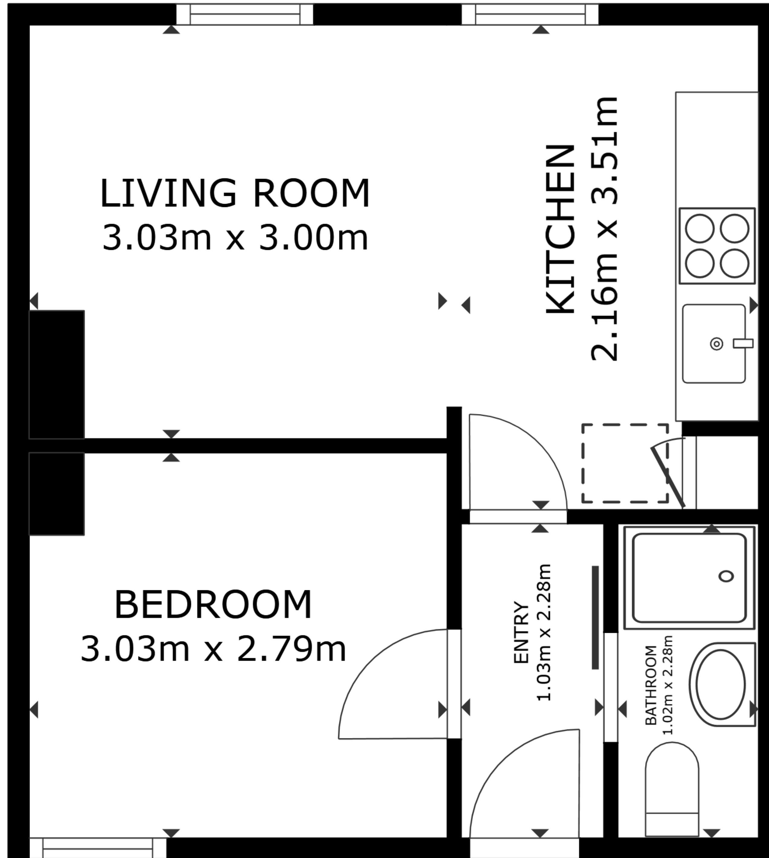
FLOOR PLAN
