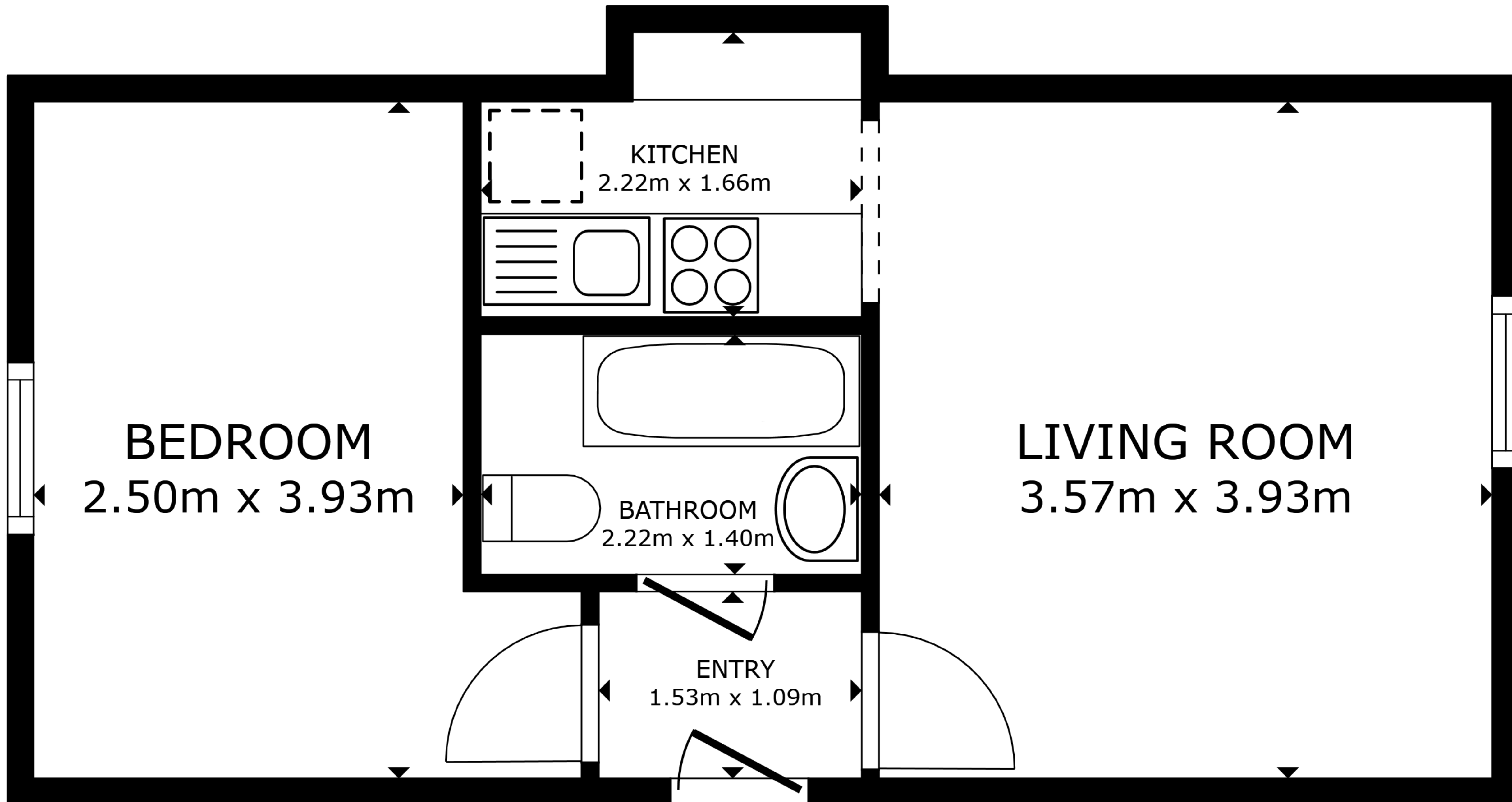
FLOOR PLAN
