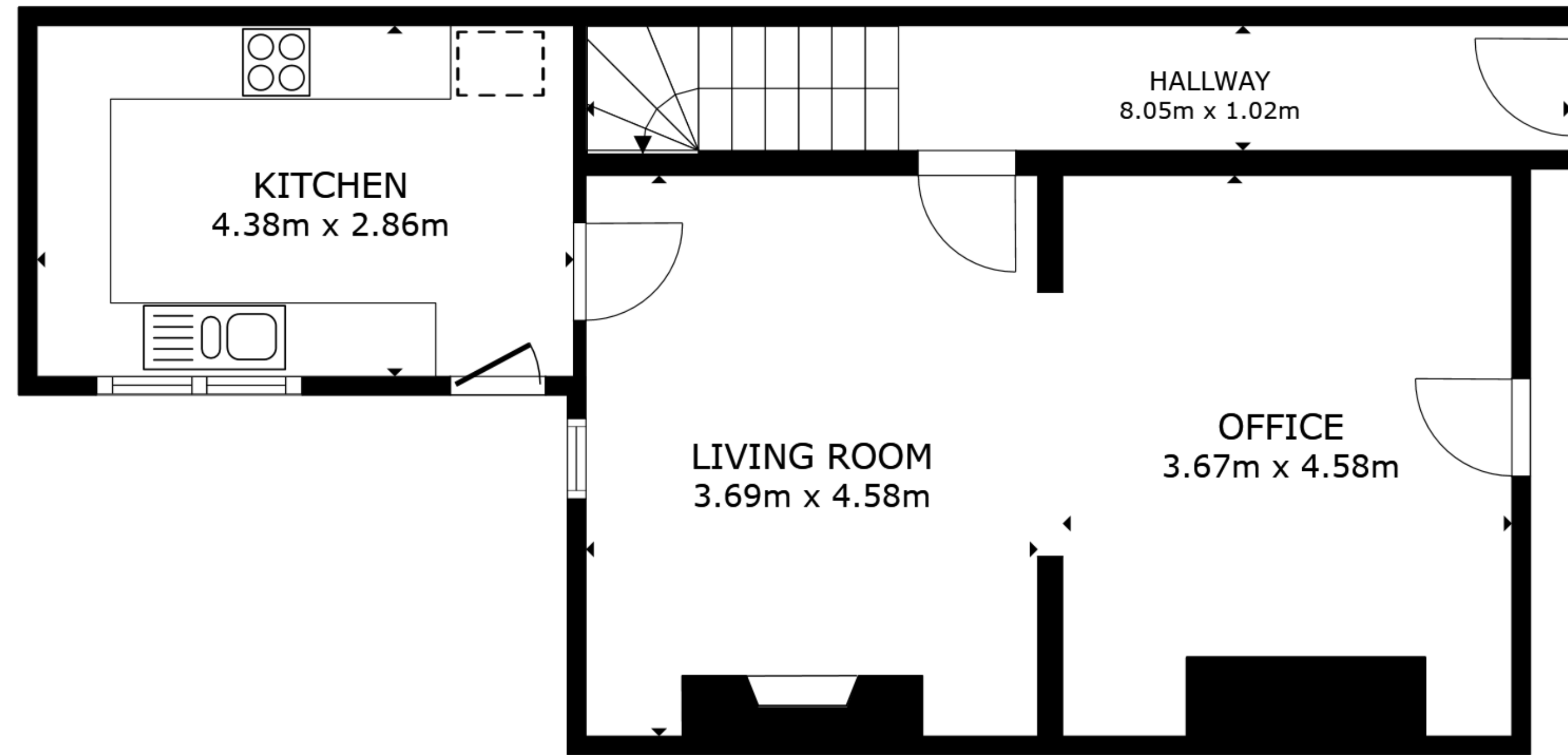
FLOOR 1
