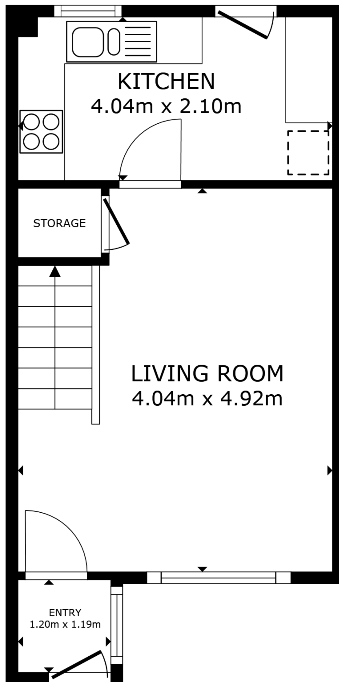
FLOOR 1
