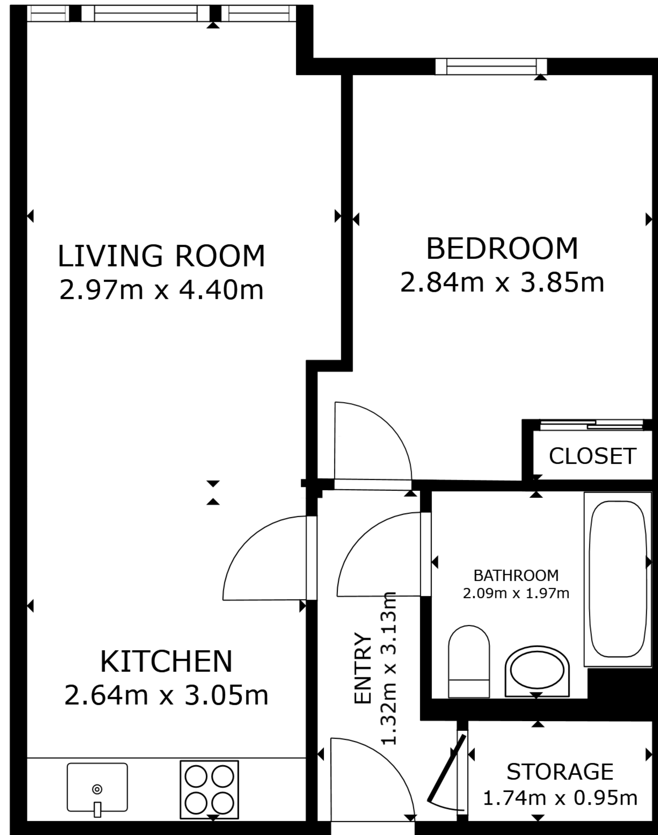
FLOOR 1
