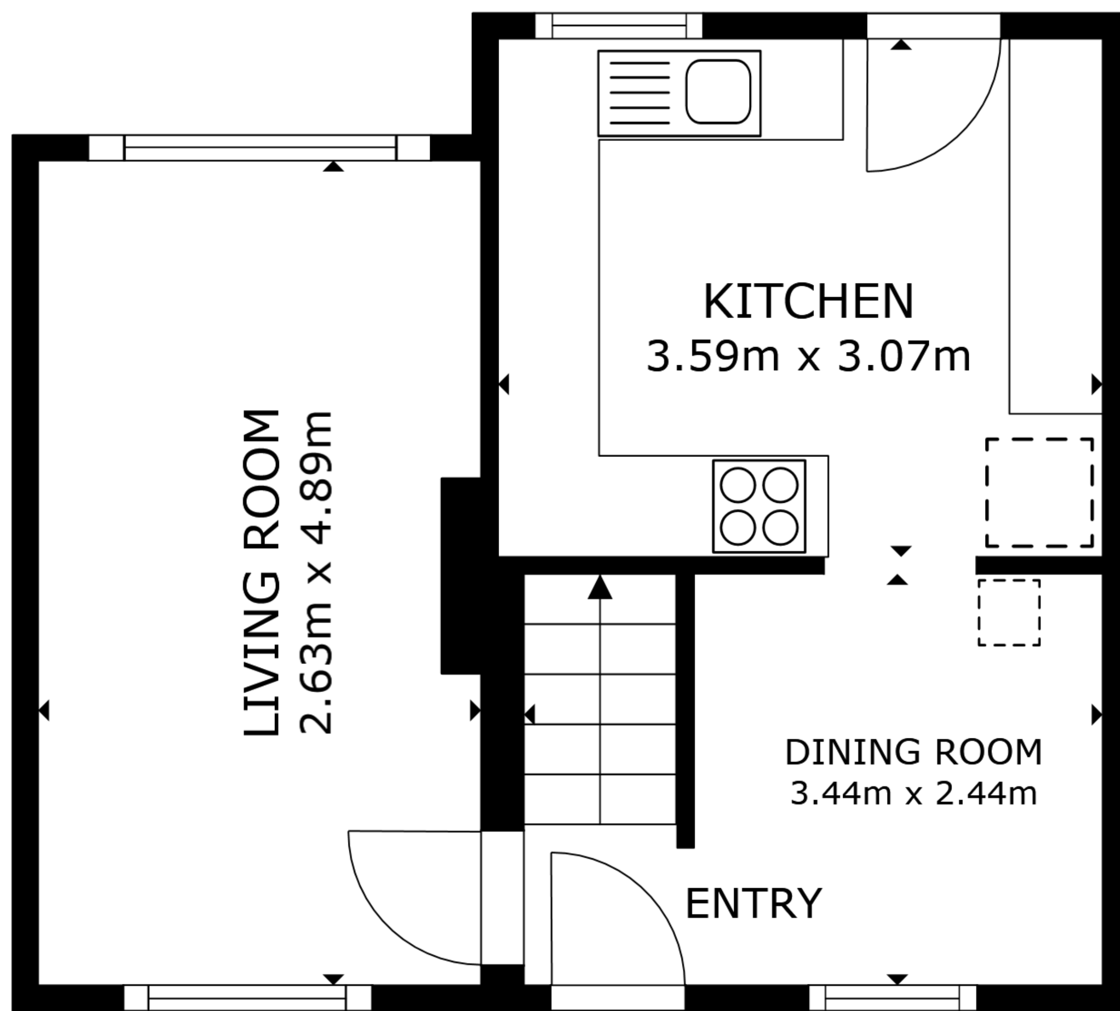
FLOOR 1
