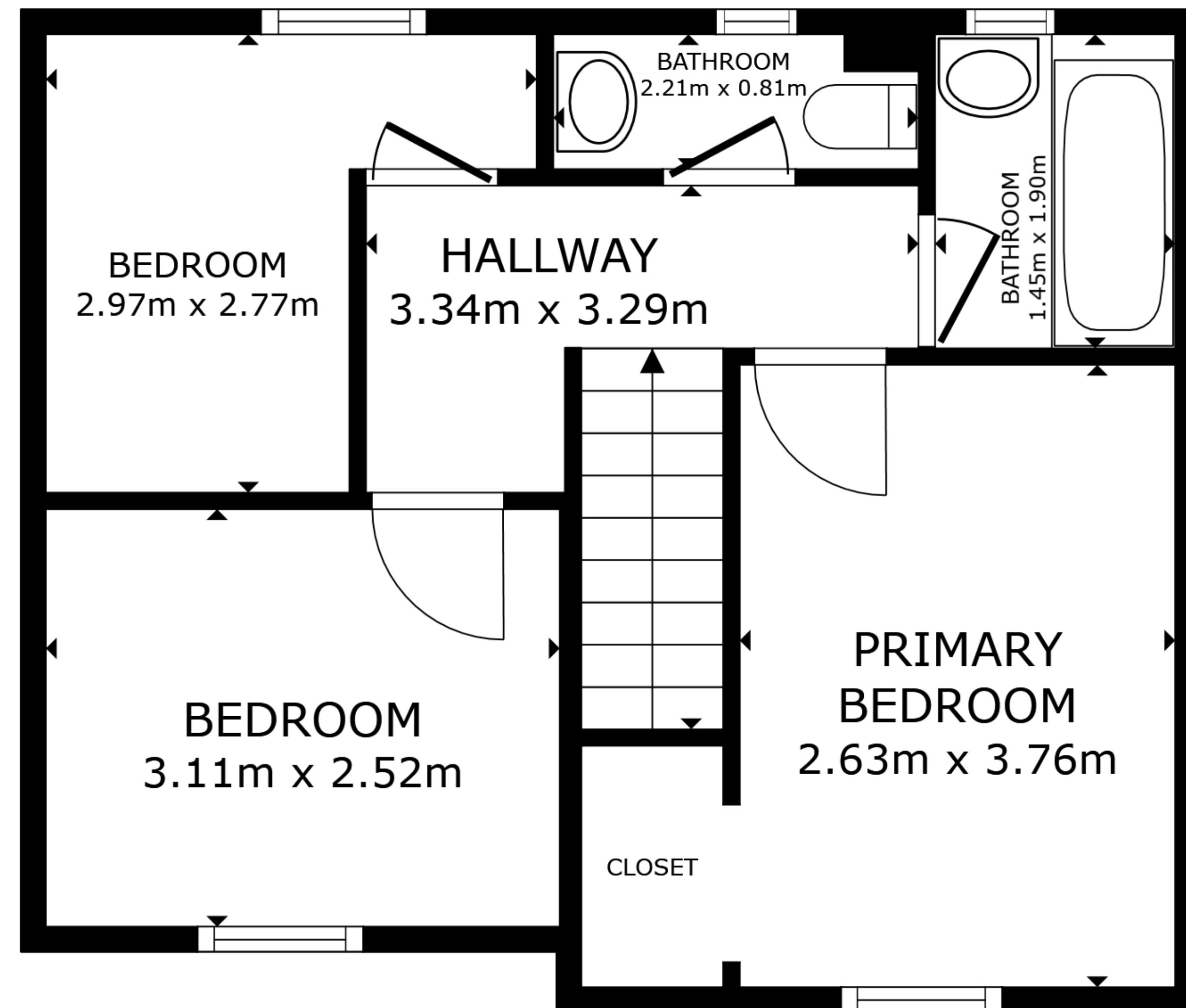
FLOOR 2
