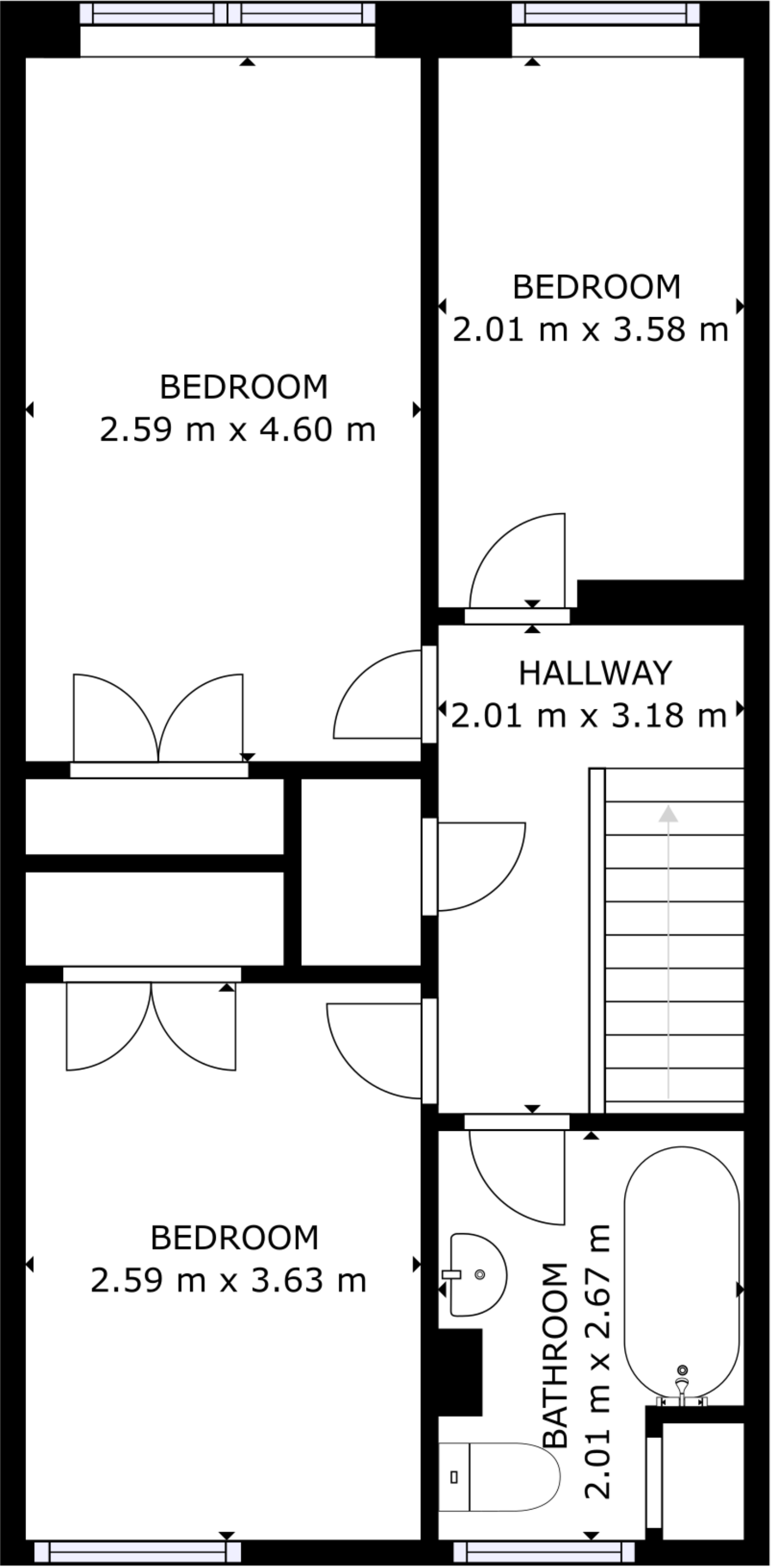
FLOOR 2
