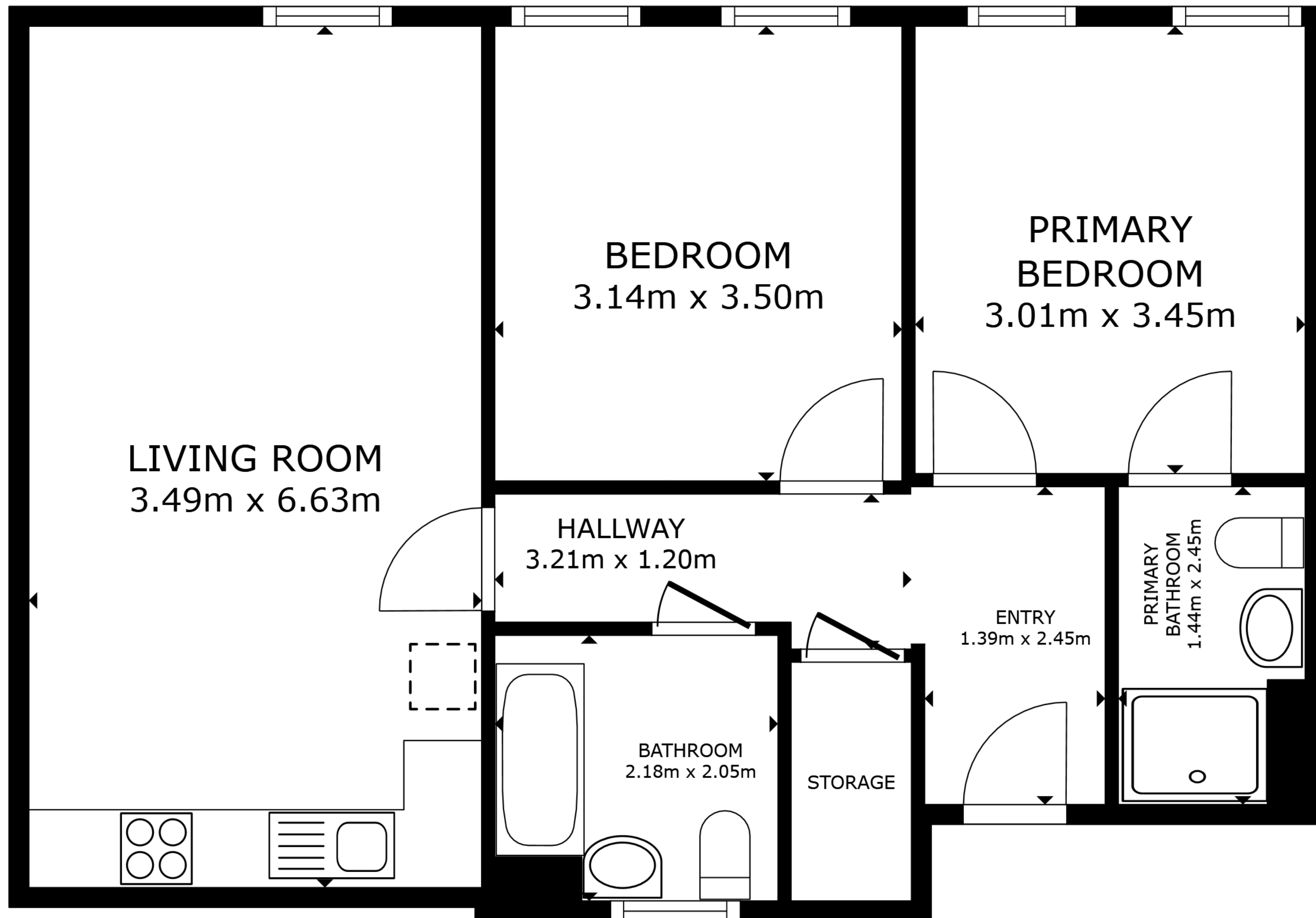
FLOOR PLAN
