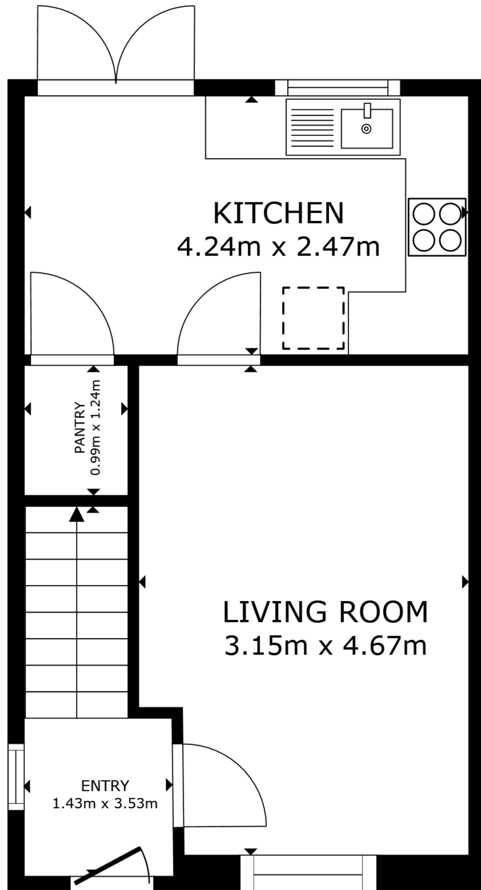
FLOOR 1
