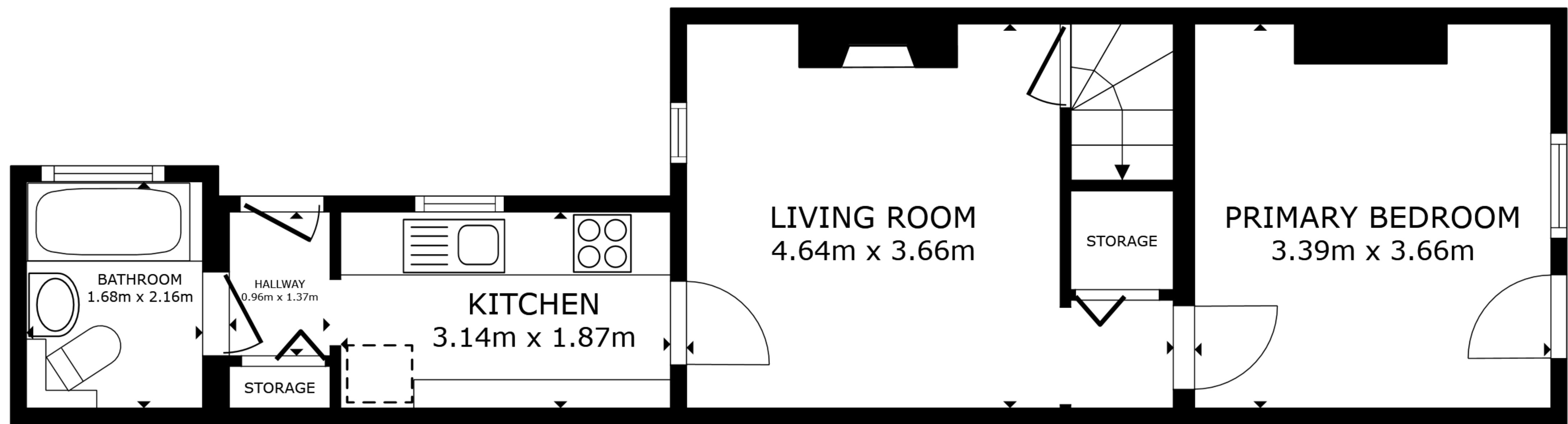
FLOOR 1
