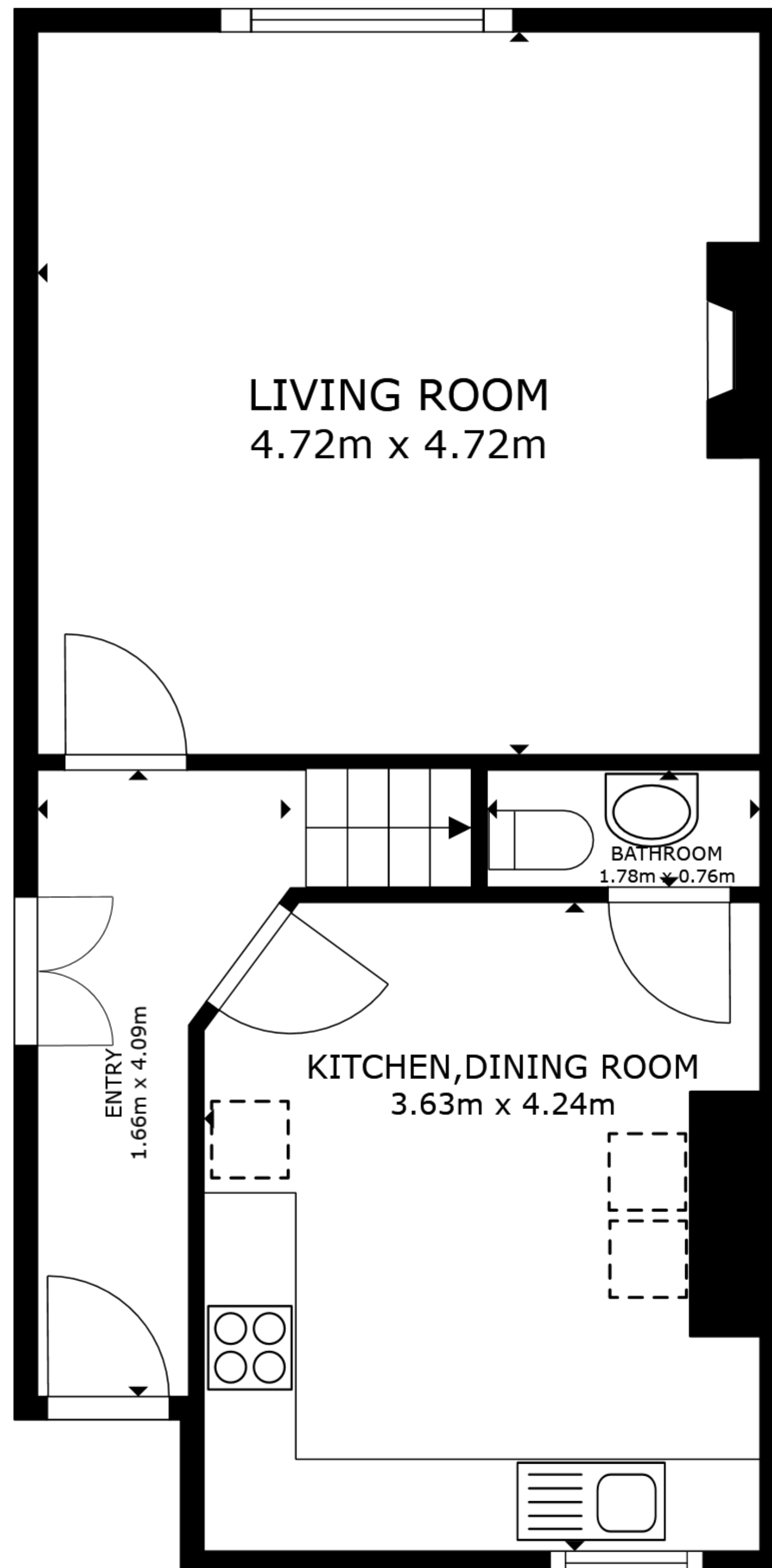
FLOOR 1
