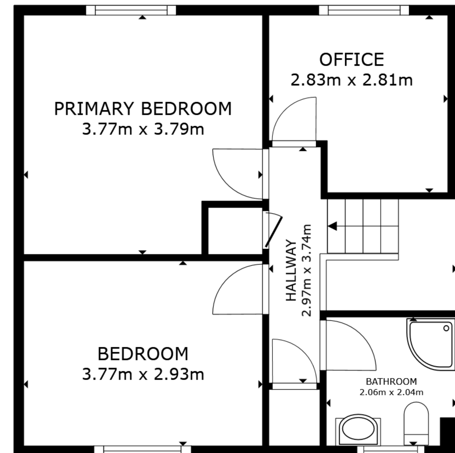
FLOOR 2
