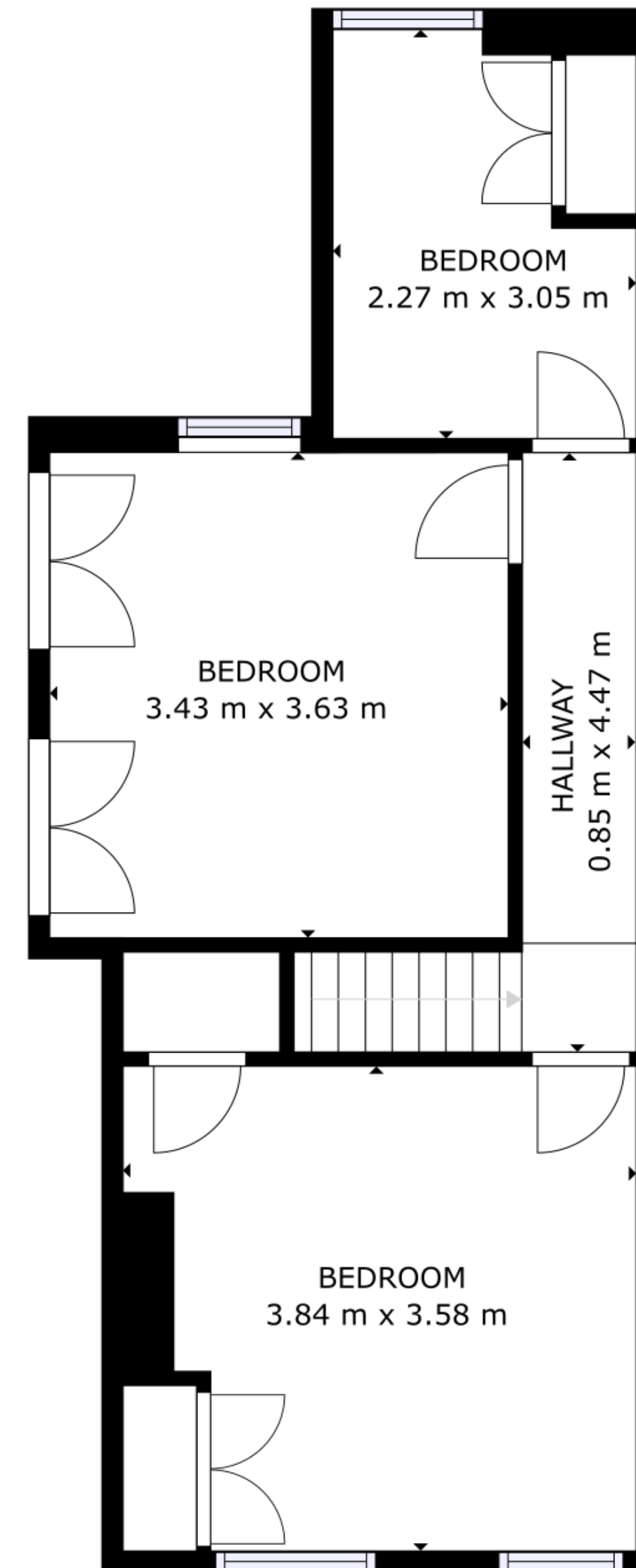
FLOOR 2
