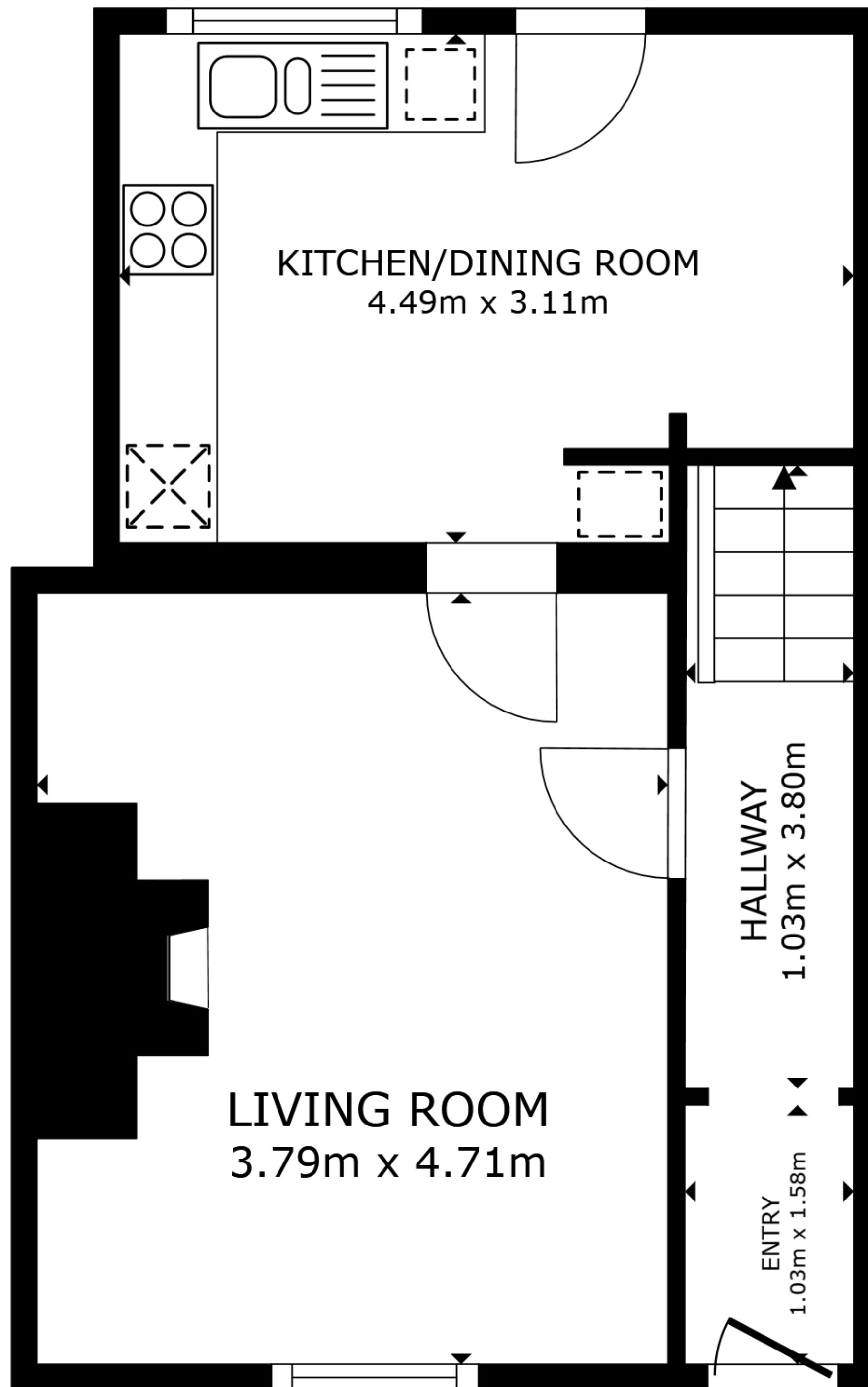
FLOOR 1
