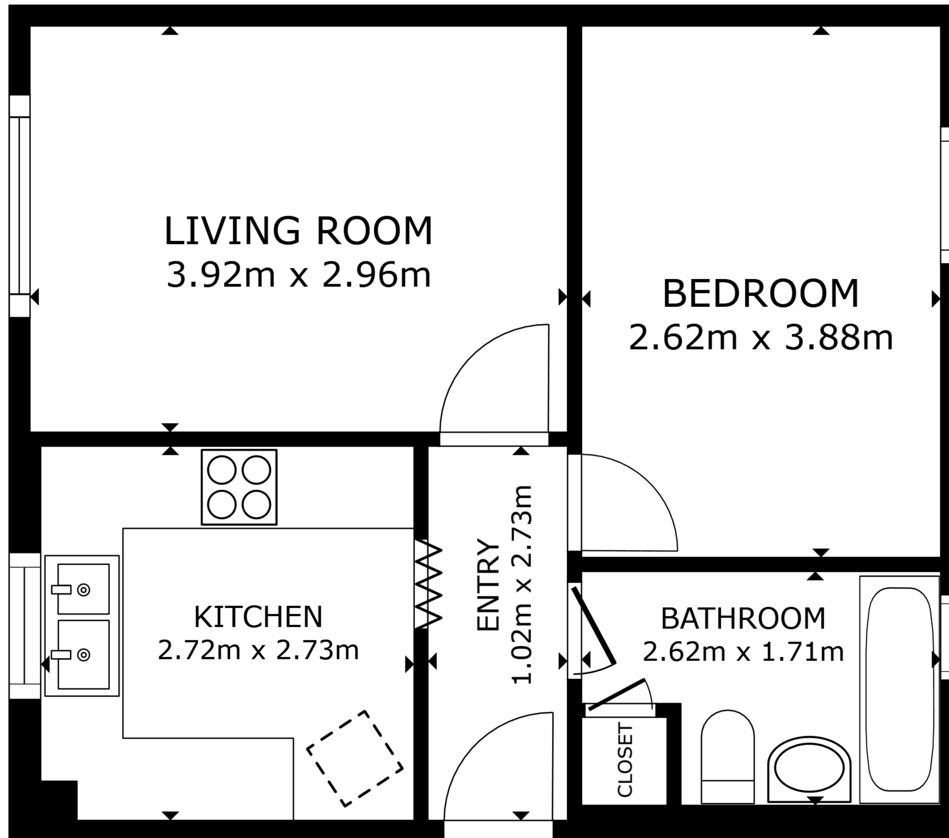
FLOOR PLAN
