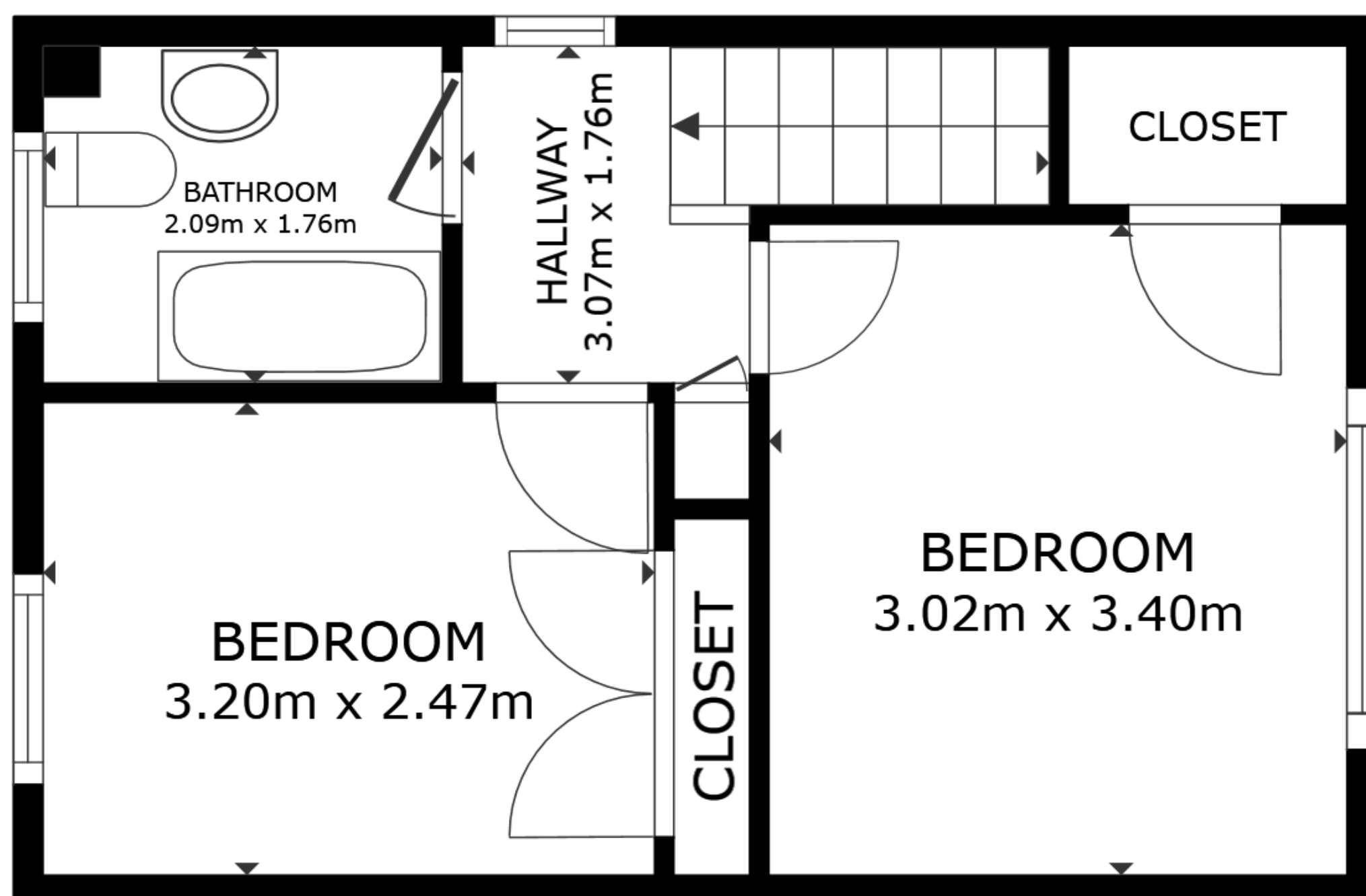
FLOOR 3
