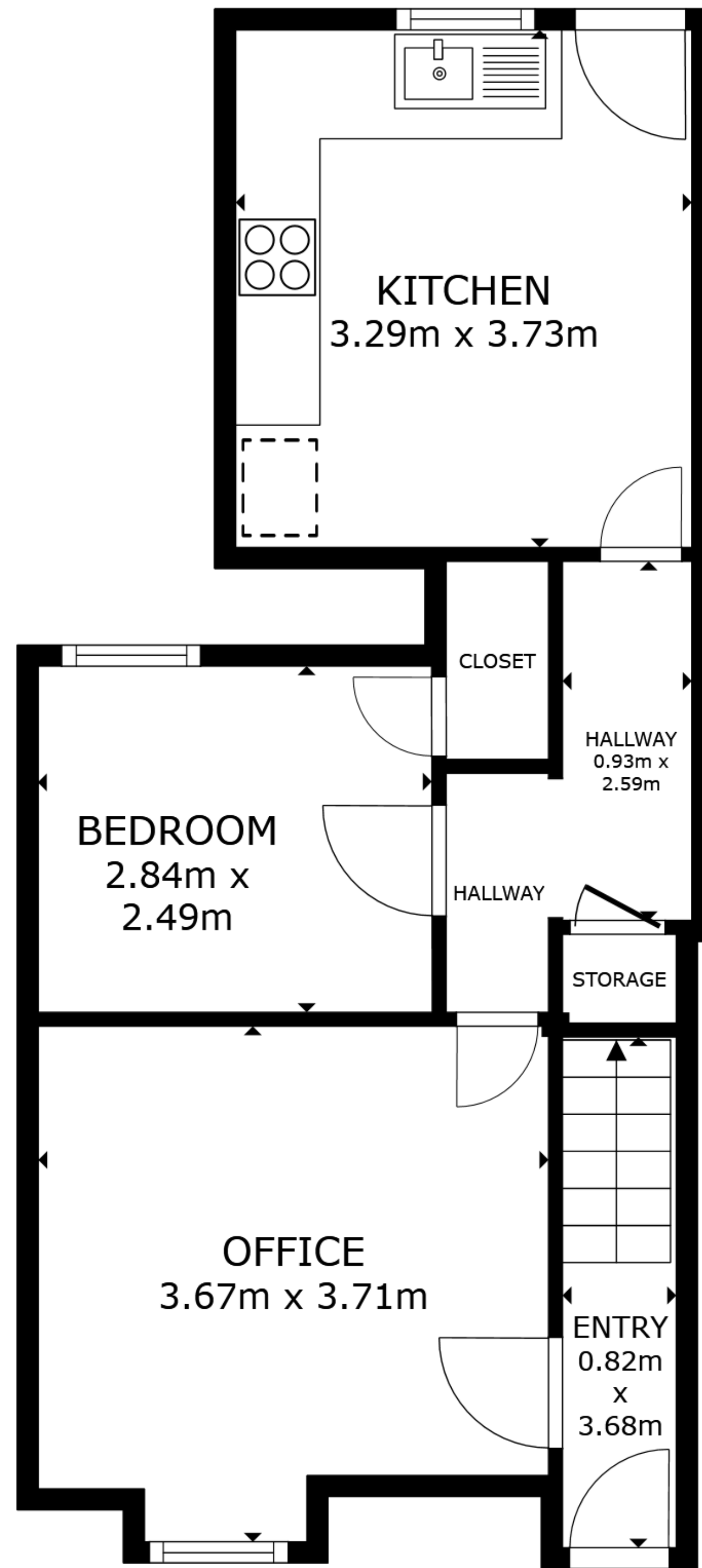
FLOOR 1
