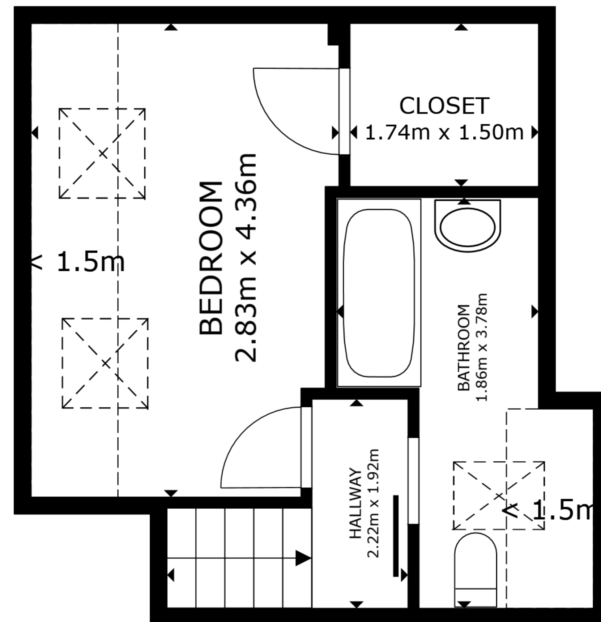
FLOOR 2
