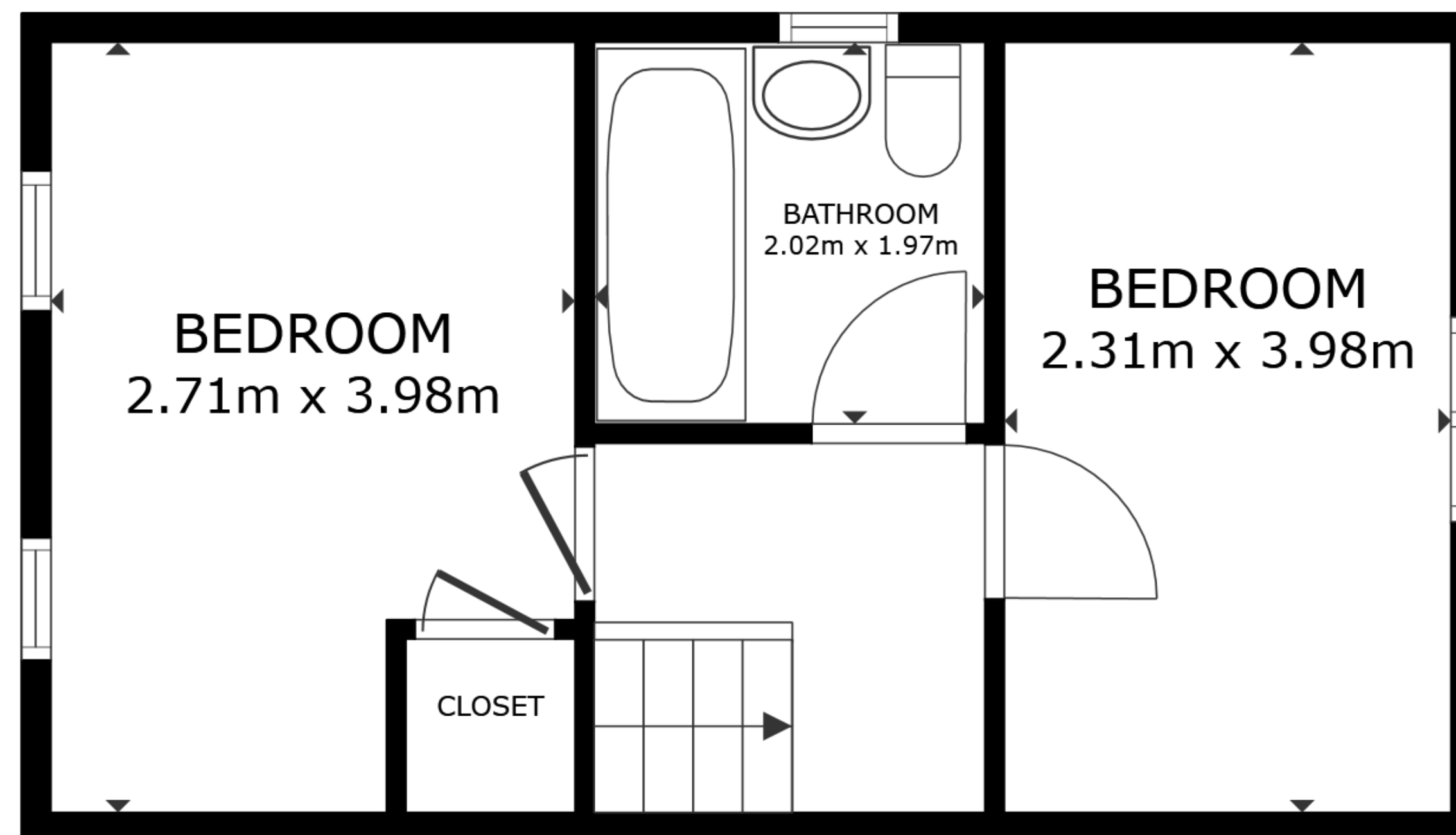
FLOOR 2
