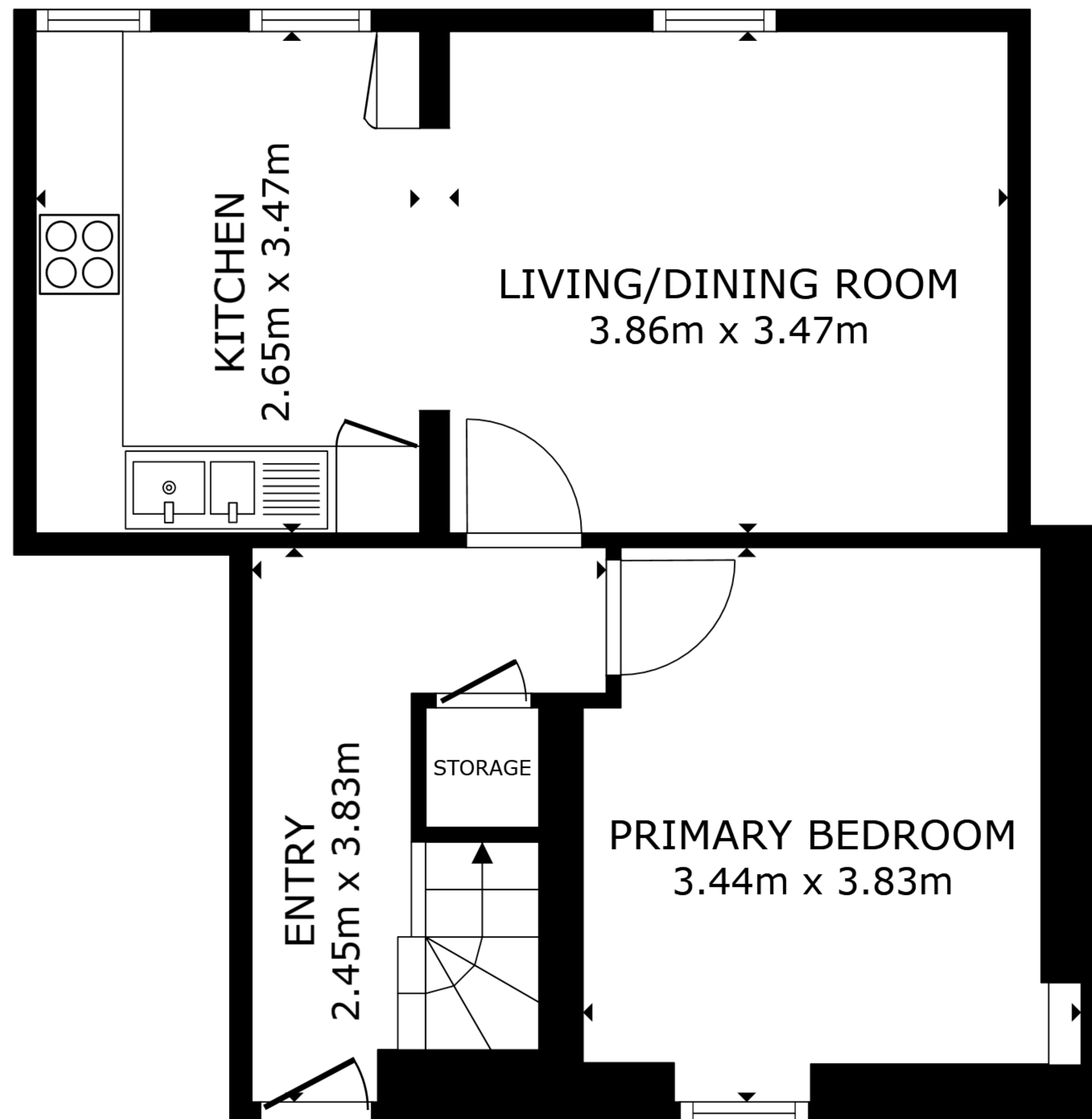
FLOOR 1
