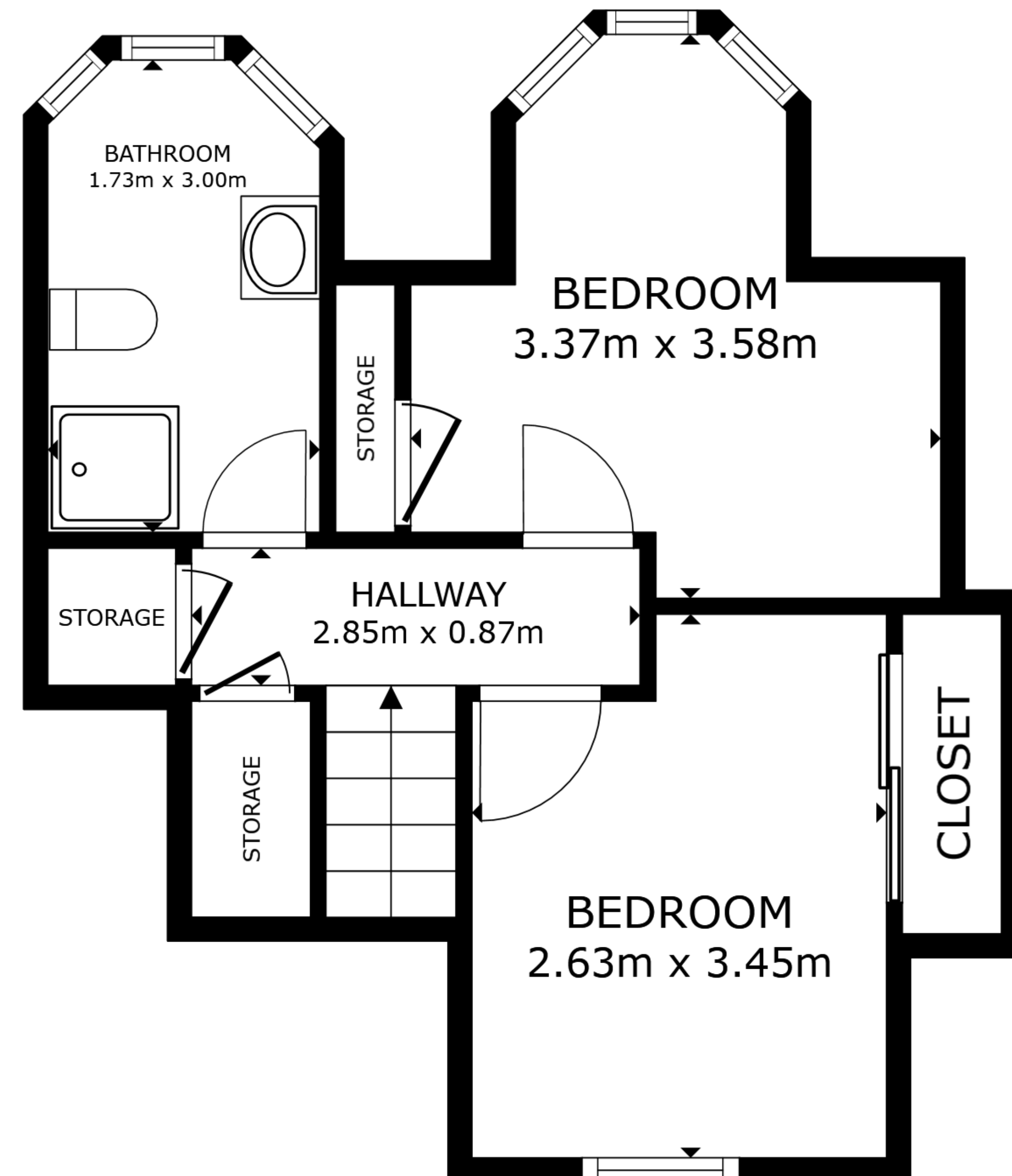
FLOOR 2
