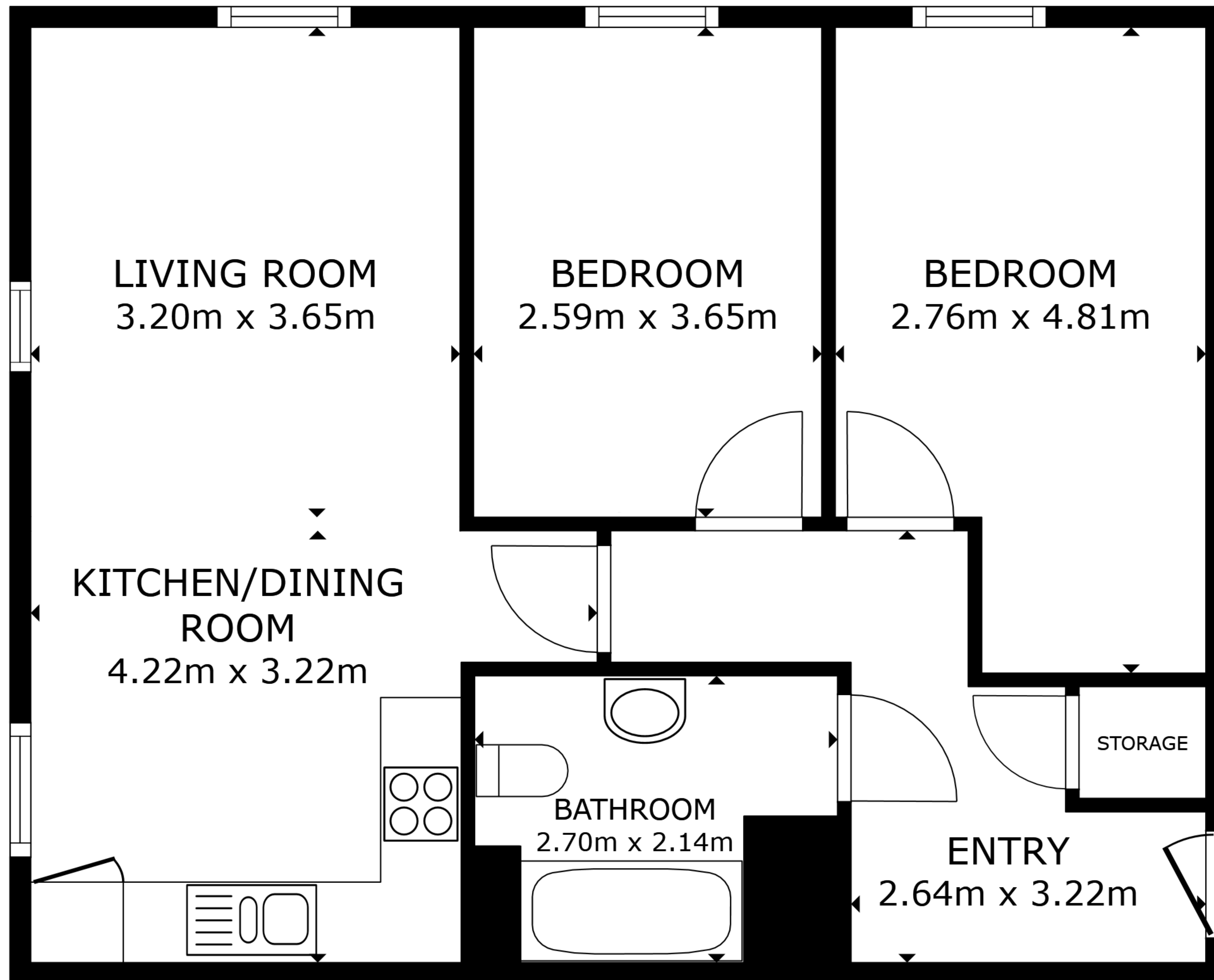
FLOOR PLAN
