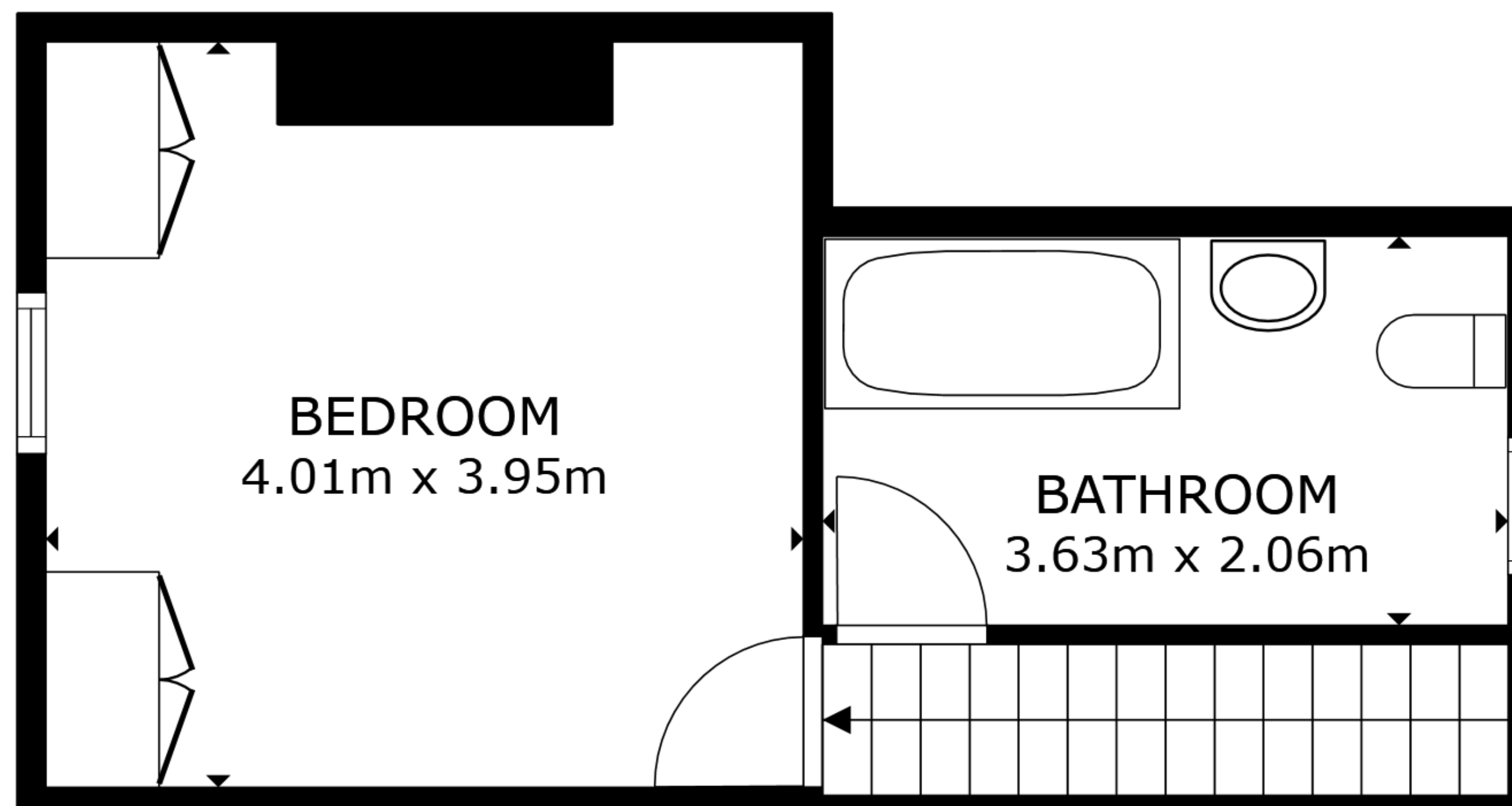
FLOOR 2
