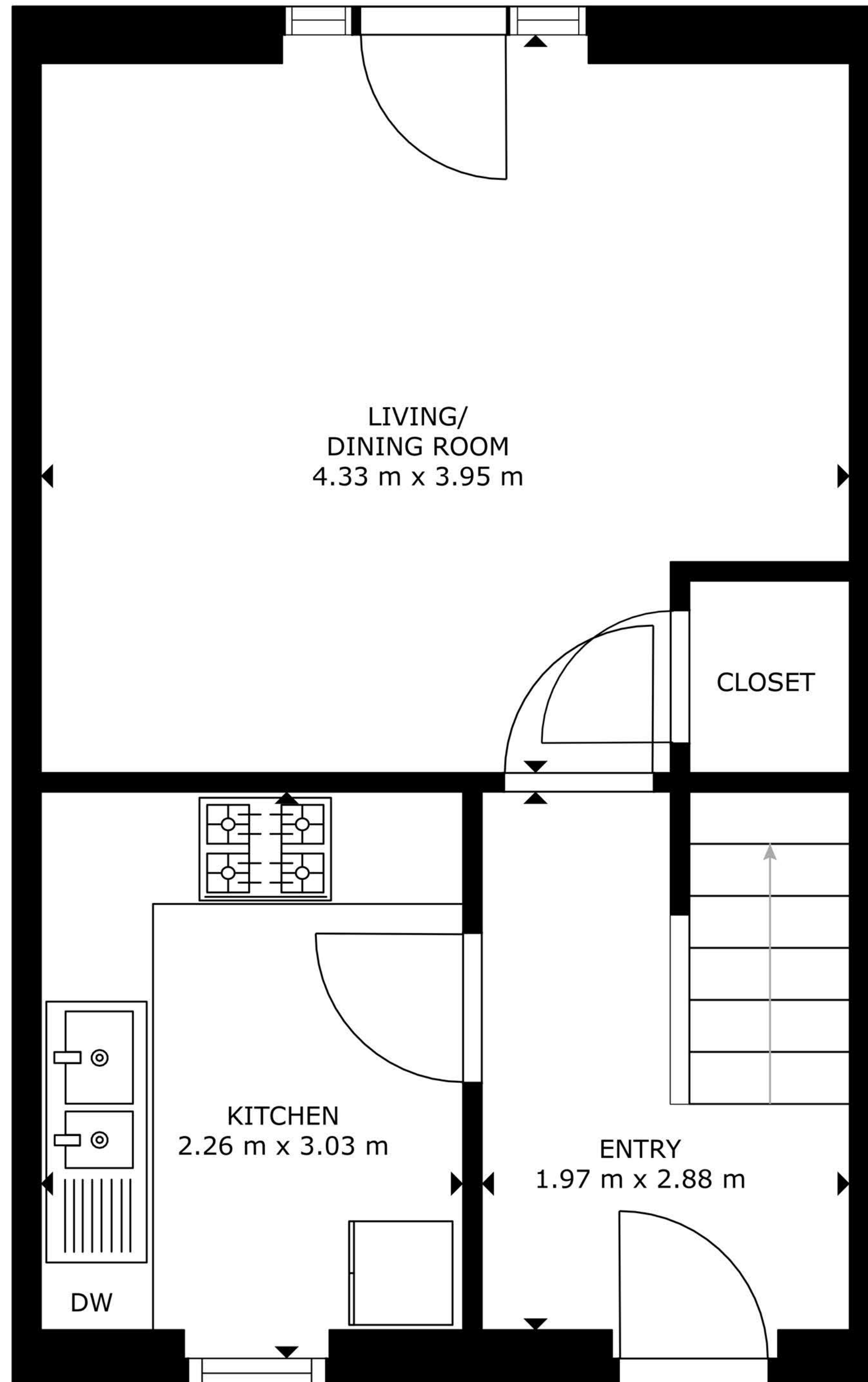
FLOOR 1
