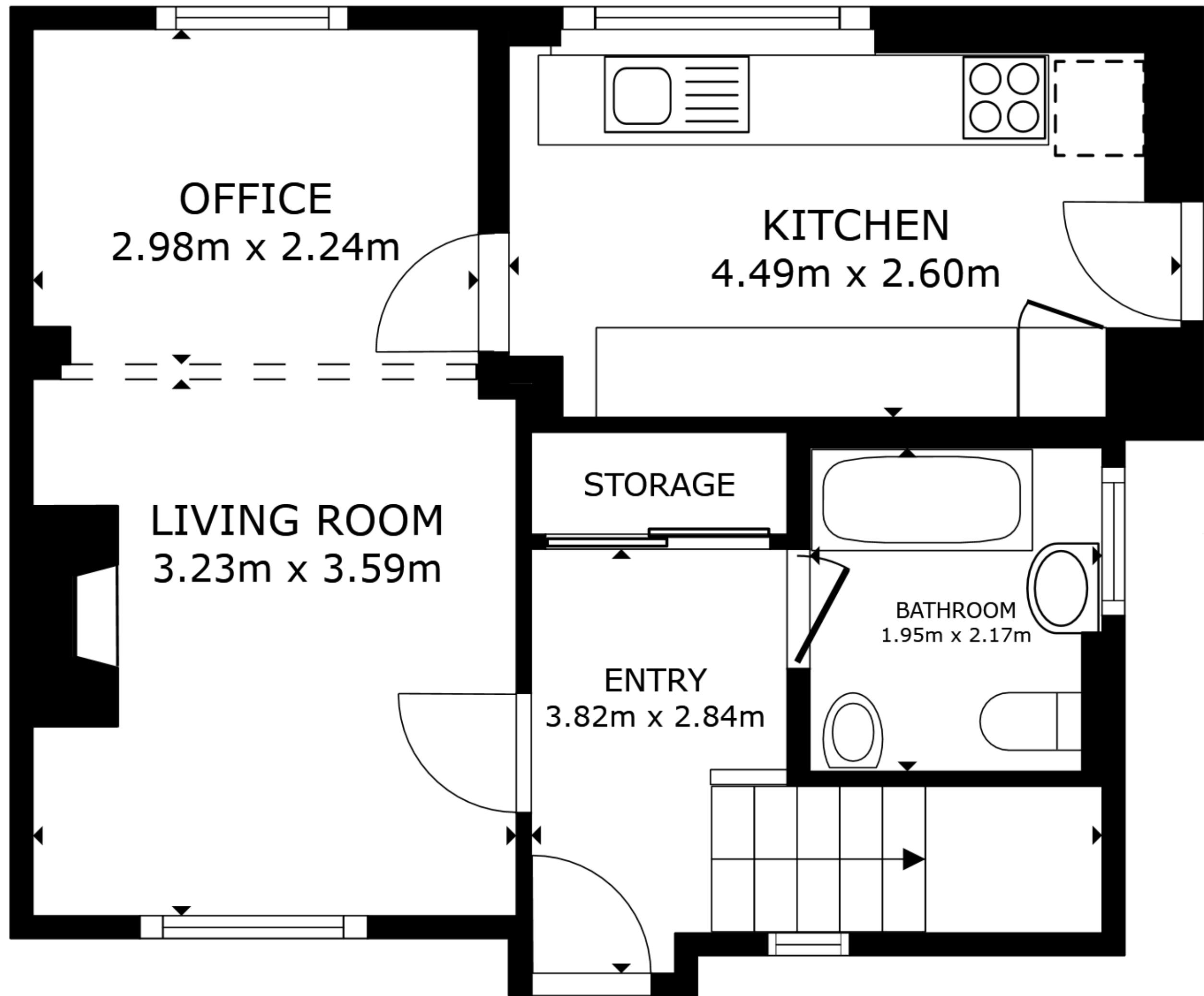
FLOOR 1
